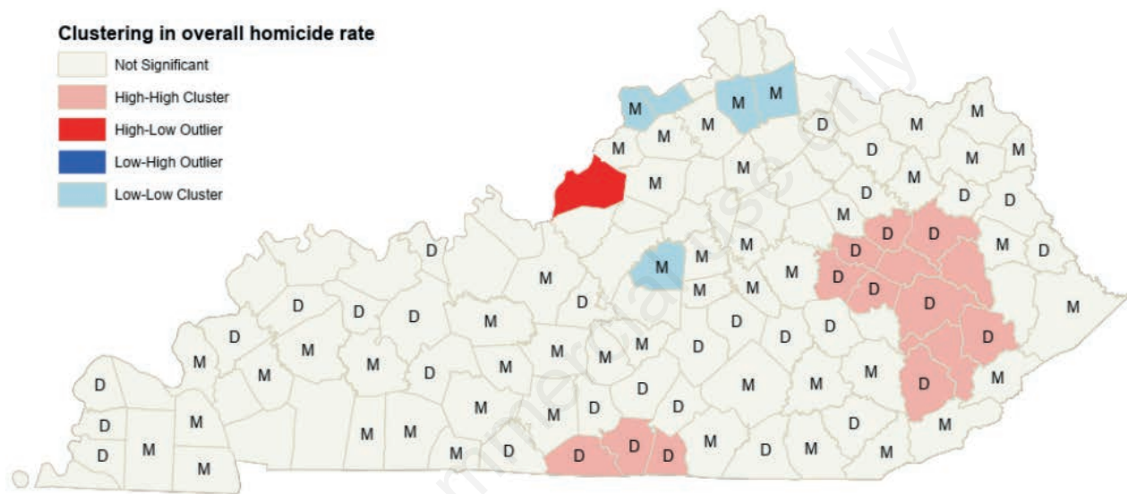
Figure 1. Cluster and outlier analysis of homicide rates in Kentucky, 2005-2012.
