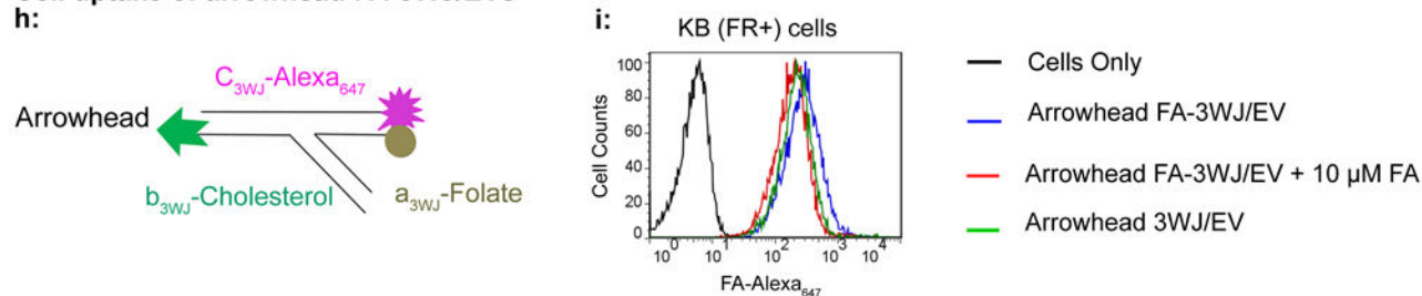
Figure 2. Comparison of the role between arrow-head and arrow-tail 3WJ (a–b) Illustration showing the difference between arrow-head and arrow-tail display. (c) Syner gel to test arrow-head and arrow-tail Alexa 647 -3WJ/EV degradation by RNase in FBS. The gel was imaged at Alexa 647 channel (d) and the bands were quantified by Image J. (e–i) Assay to compare cell binding of folate-3WJ arrow-tail (e–g) and arrow-head (h–i) on folate receptor positive and negative cells.
