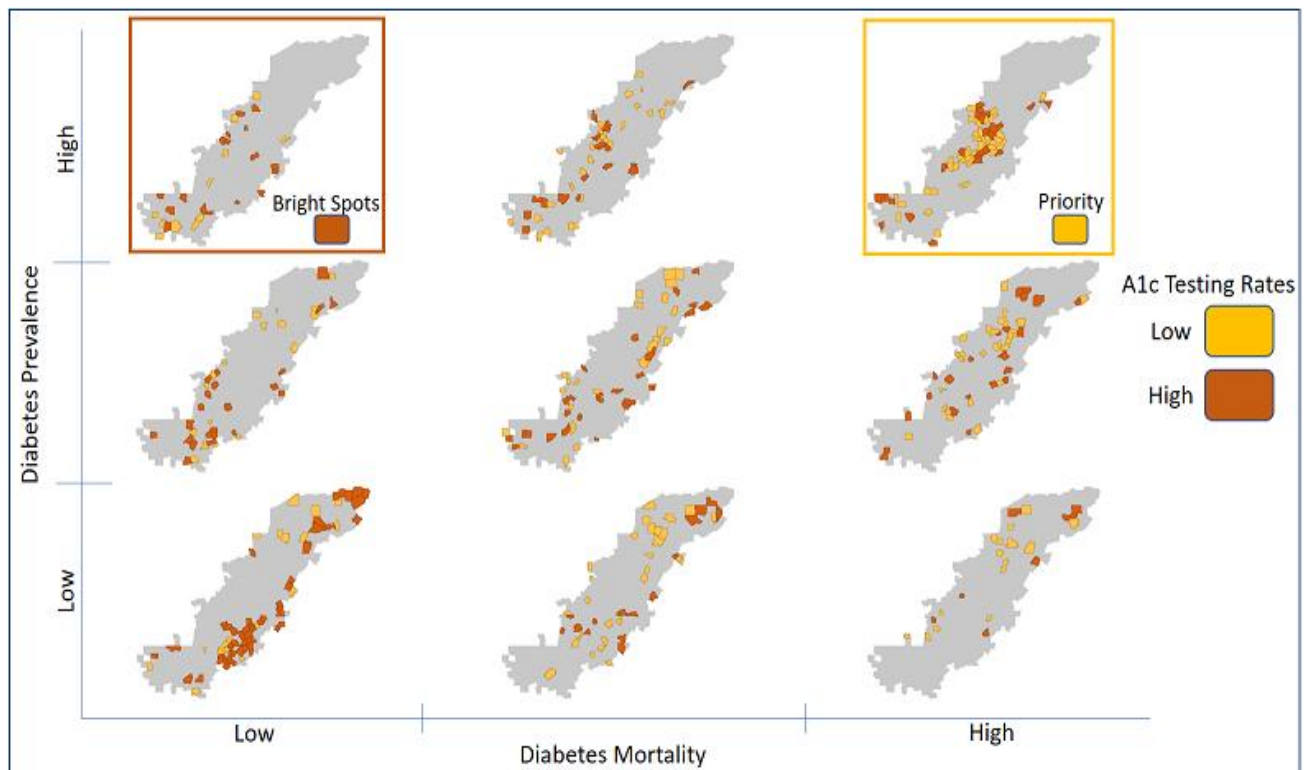
Figure 1. HbA1c testing rates, conditioned on diabetes prevalence and mortality
