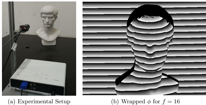
Figure 5. Experimental setup and wrapped phase
