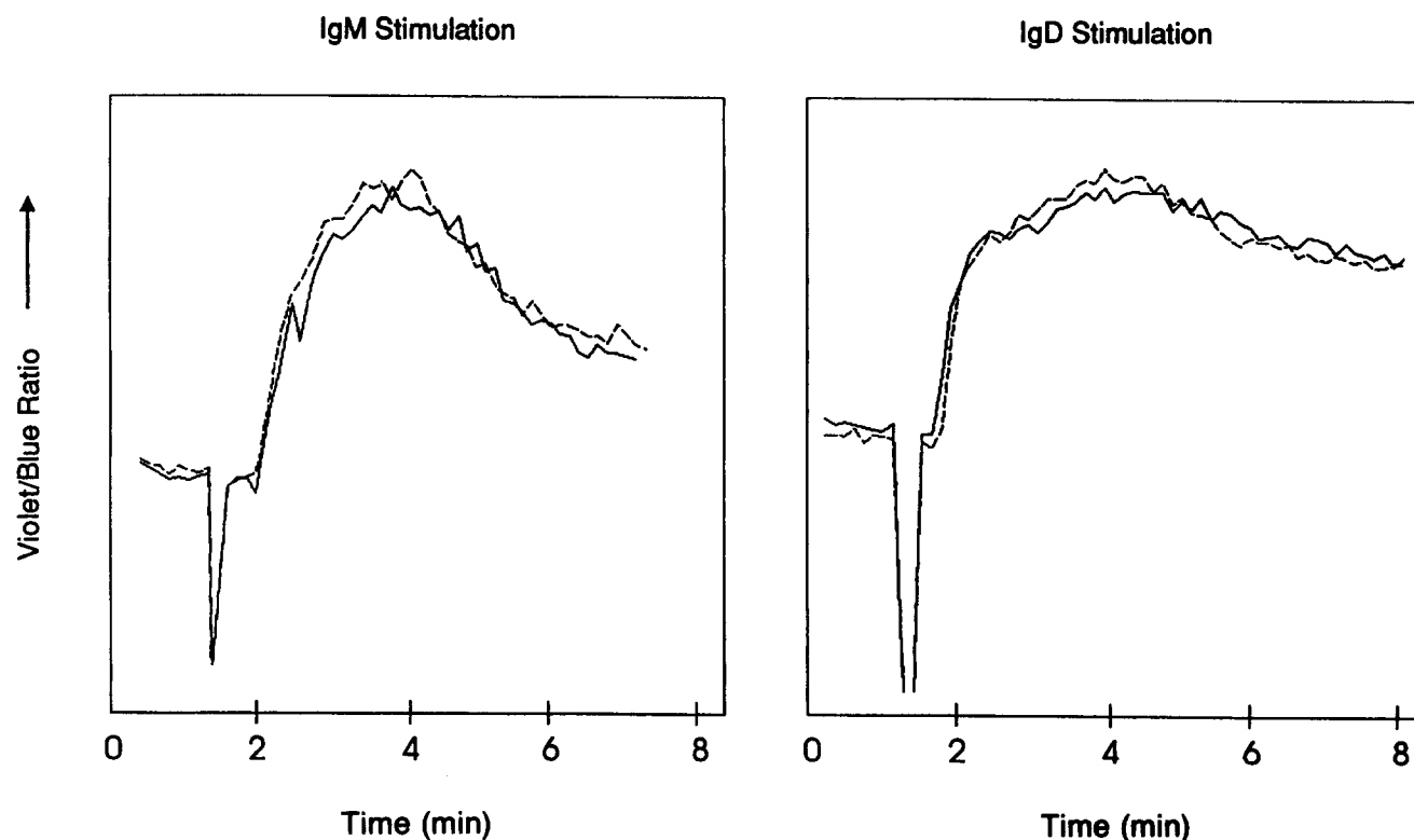
Figure 3. Ca 2+ accumulation in fyn Tnull splenocytes. Intracellular concentrations of Ca 2+ were determined by flow cytometry of Indo1-labeled cells after stimulation with anti-IgM at 80 \mu g/ml or anti-IgD at 100 \mu g/ml. Calcium responses of B220 surface-stained populations from control (solid line) and fyn Tnull animals (dashed line) are compared.
