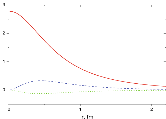
Fig. 1 Normalized wave functions of the \Sigma_c \bar{D}^* bound state with J^P = 3/2^-, T = 1/2 and the binding energy 14.6 MeV ( \Lambda = 1430 MeV). The |L = 0, S = 3/2\rangle , |L = 2, S = 1/2\rangle , and |L = 2, S = 3/2\rangle wave functions are solid, dotted, and dashed lines, respectively
