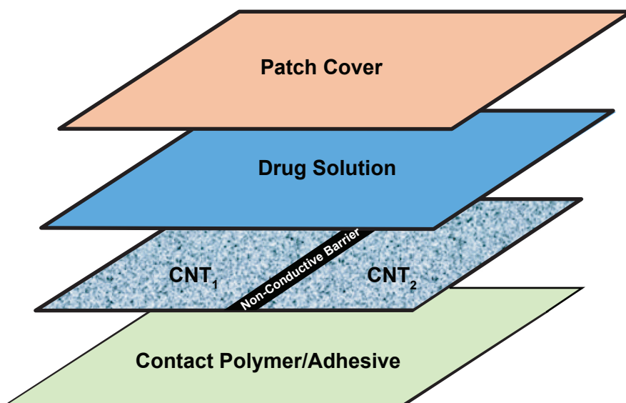
Figure 3b. Schematic of patch layering using two CNT membranes to produce three different transdermal fluxes.
