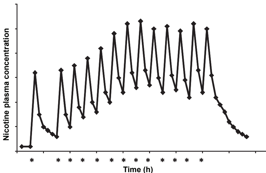
Figure 1a. Representative nicotine plasma profile of a cigarette smoker. Asterisks indicate the smoking of a cigarette.
