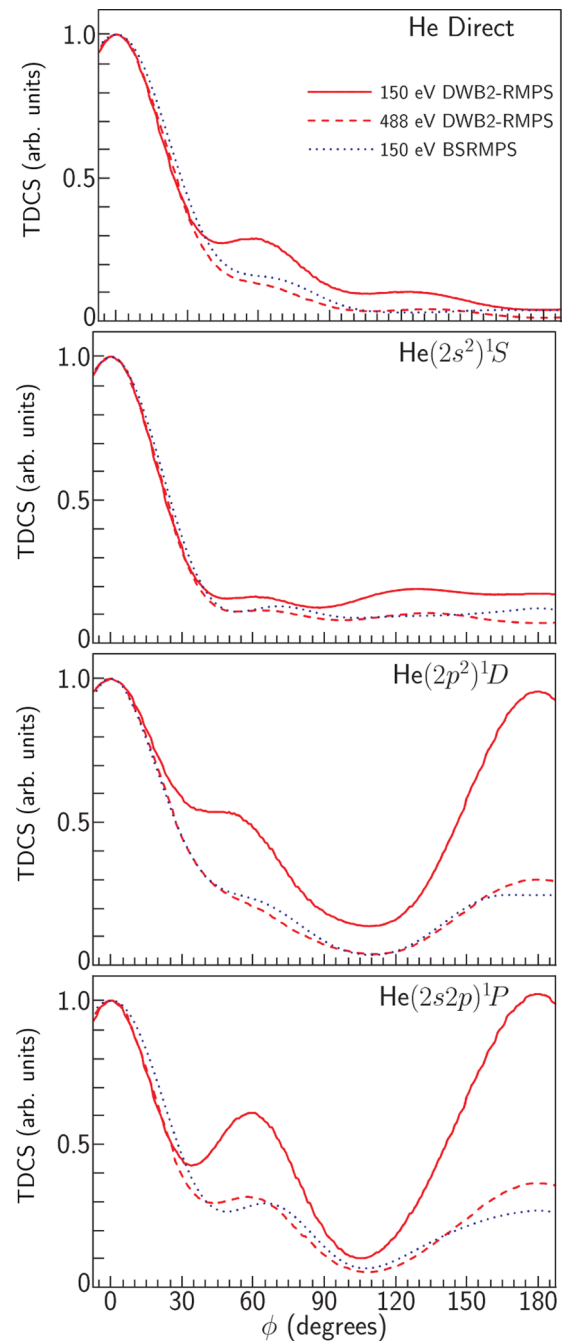
FIG. 3. DWB2-RMPS calculations of the ( e,2e ) ejected-electron angular distributions for 150 eV and 488 eV incident energy compared with the 150 eV BSRMPS calculations. All calculations are normalized in the binary peak. See text for details.
