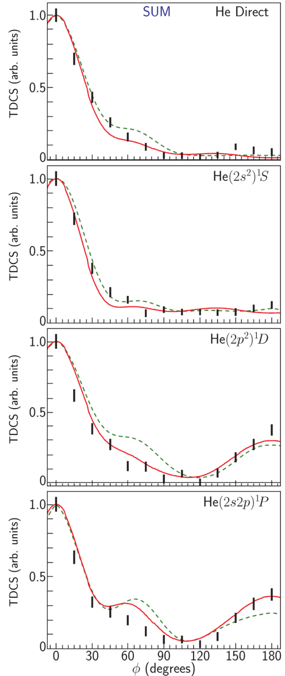
FIG. 6. Weighted sum of the experimental data for 150, 120, and 100 eV incident-electron energies (see text), compared with the DWB2-RMPS calculation for 488 eV (solid line) and the BSRMPS calculation for 120 eV (dashed line). Theory and experiment are normalized to unity at \phi = 0 .
