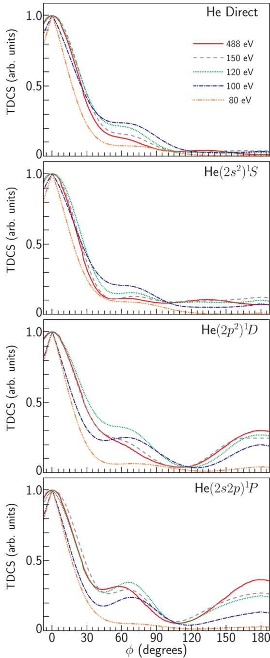
FIG. 2. Calculated ( e,2e ) ejected-electron angular distributions described in the text. The incident-electron energies correspond to the experiments described below. The 488 eV is a DWB2-RMPS calculation and the remainder are BSRMPS calculations.
