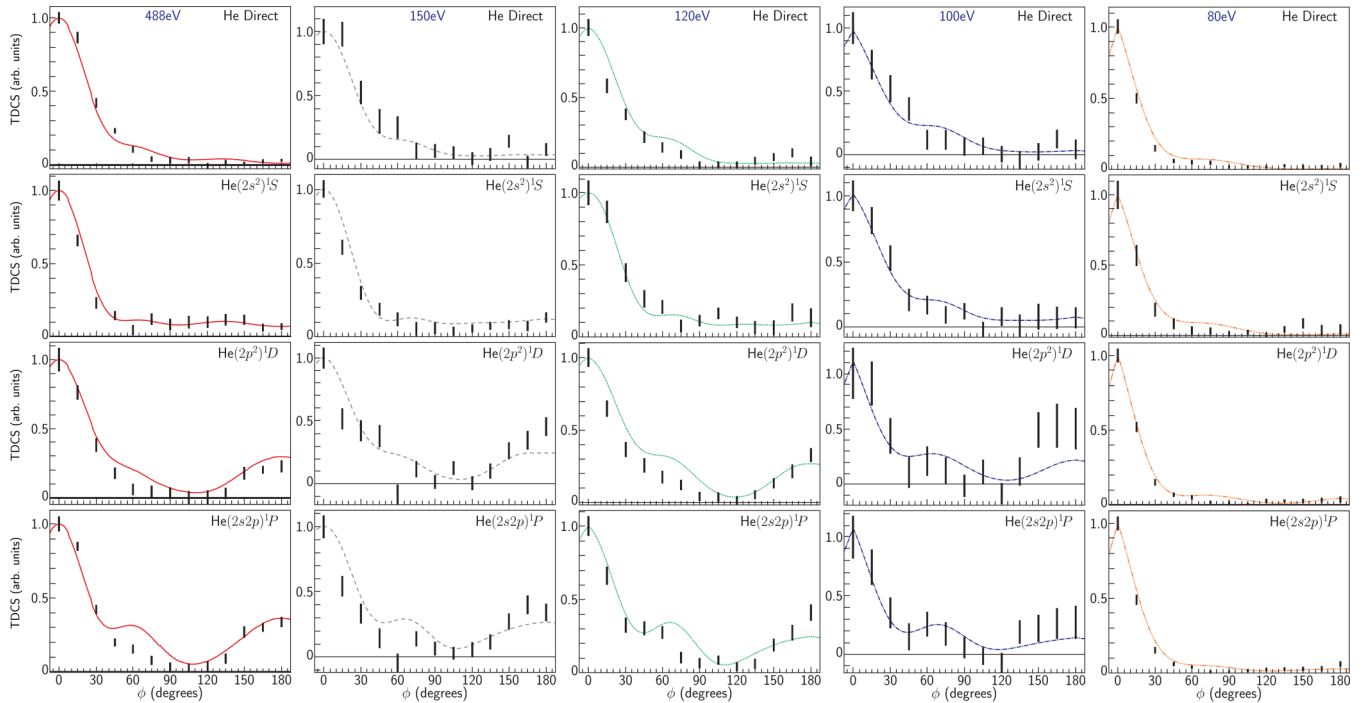
FIG. 5. Out-of-plane ( e,2e ) angular distributions, for helium direct ionization and the (2s^2)^1S , (2p^2)^1D , and (2s2p)^1P autoionizing resonances, for 488, 150, 120, 100, and 80 eV incident-electron energy. The corresponding scattering angles are given in Table I. The vertical bars represent the experimental results and indicate the statistical errors. The theoretical curves are those from Fig. 2. Theory and experiment are normalized to unity at \phi = 0 .
