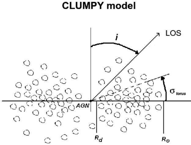
Figure 7. CLUMPY dusty torus geometry as described in Nenkova et al. (2008a,b). The radial extent of the torus is defined by the ratio between the outer radius R_o and the dust sublimation radius R_d , Y = R_o/R_d , with Y a free parameter. All clouds are assumed to have the same optical depth \tau_v . The angular width is given by \sigma , and N_{\text{LOS}} is the mean number of clouds found along a LOS at angle i .
