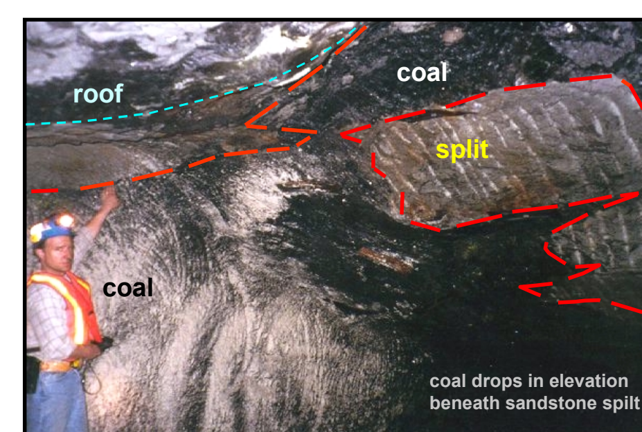
Figure 12. Split and over-thickened coal along outcrop margin.
