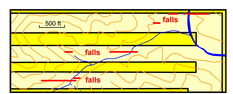
Figure 7. Roof falls (red) beneath low cover in an underground mine (light yellow). Blue lines are streams and orange lines are surface contours (after Greb and Popp, 1999, Fig. 13A).
