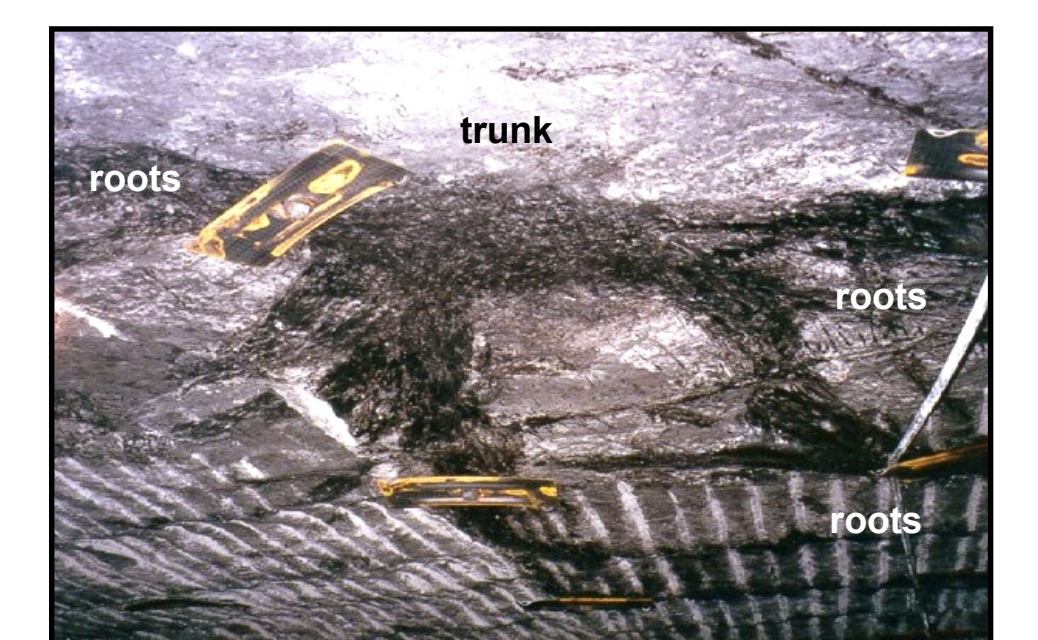
Figure 22. Kettlebottom in shale roof above Lower Elkhorn coal.
