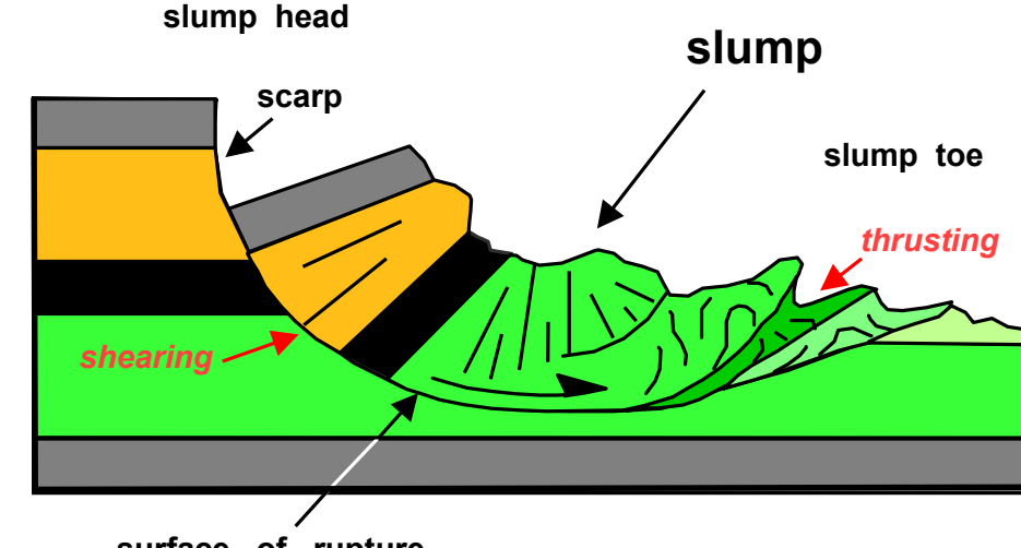
Figure 15. Schematic section through a slump.
