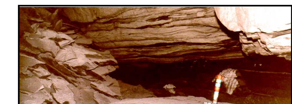
Figure 17. Stackrock strata in roof fall above Lower Elkhorn coal.
