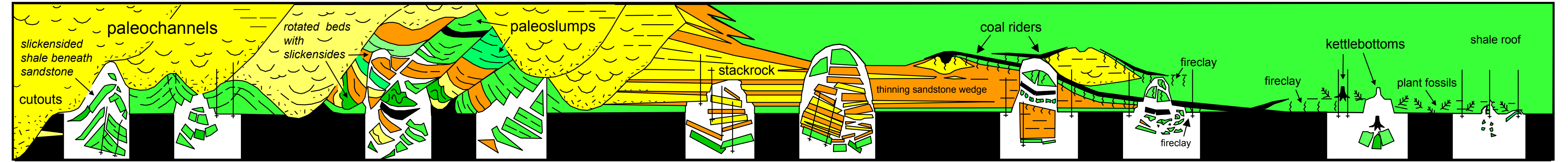
Figure 8. Schematic diagram showing the types of lateral variation seen in roof rocks, and inherent mining obstacles associated with each, above the Lower Elkhorn coal bed. Rates of variation are variable, which is why no scale is inferred.
