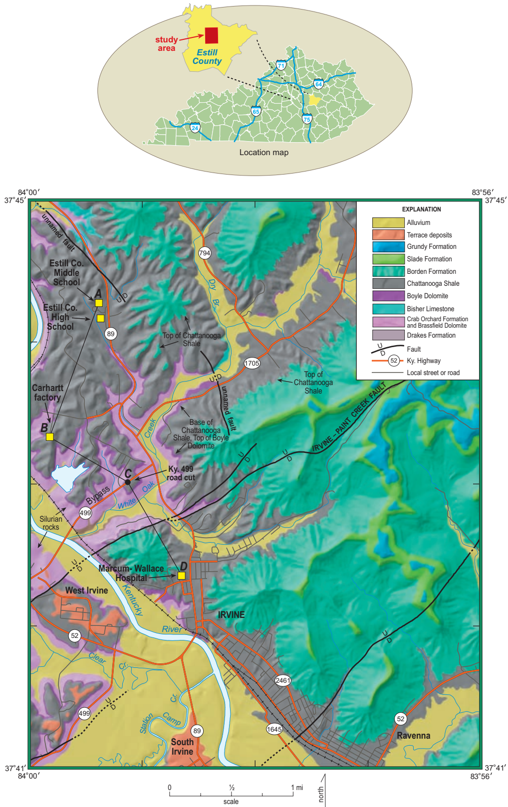
Figure 1. Geology of the North Irvine area, Estill County, Ky. Locations of buildings with foundations in the lower part of the Chattanooga Shale, which have had significant foundation structural problems, are shown. Compiled from Morris and Curl (2000).
