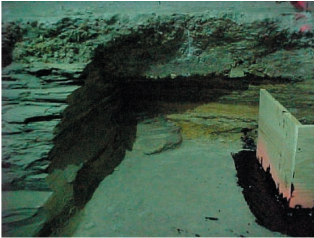
Figure 17. Cleats with copiapite in shale subcrop beneath the middle school, along with newly constructed concrete column forms.
