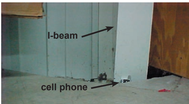
Figure 24. Heaved floor adjacent to load-bearing wall on main floor of the Carhartt factory. Note the top of a cell phone near the I-beam, which shows that the main floor was heaved upward about 4 in.
