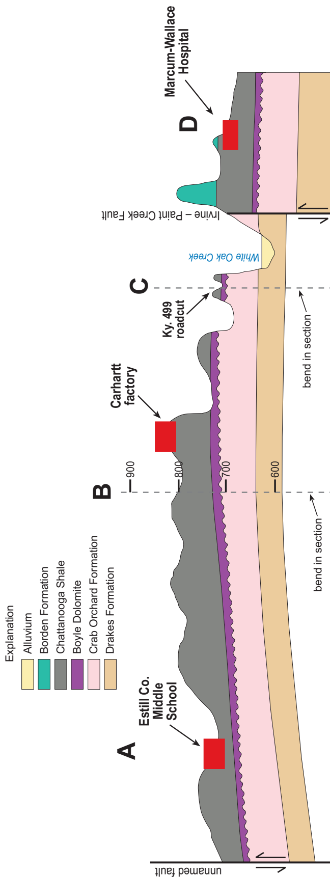
Figure 2. Cross section showing locations of buildings and roadways and position of pyrite zones in the Chattanooga Shale.
