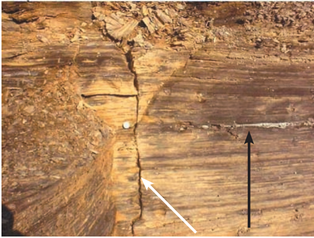
Figure 9. Cleat fractures (white arrow) and pyrite nodule zone (black arrow) in Chattanooga Shale at the middle school.
