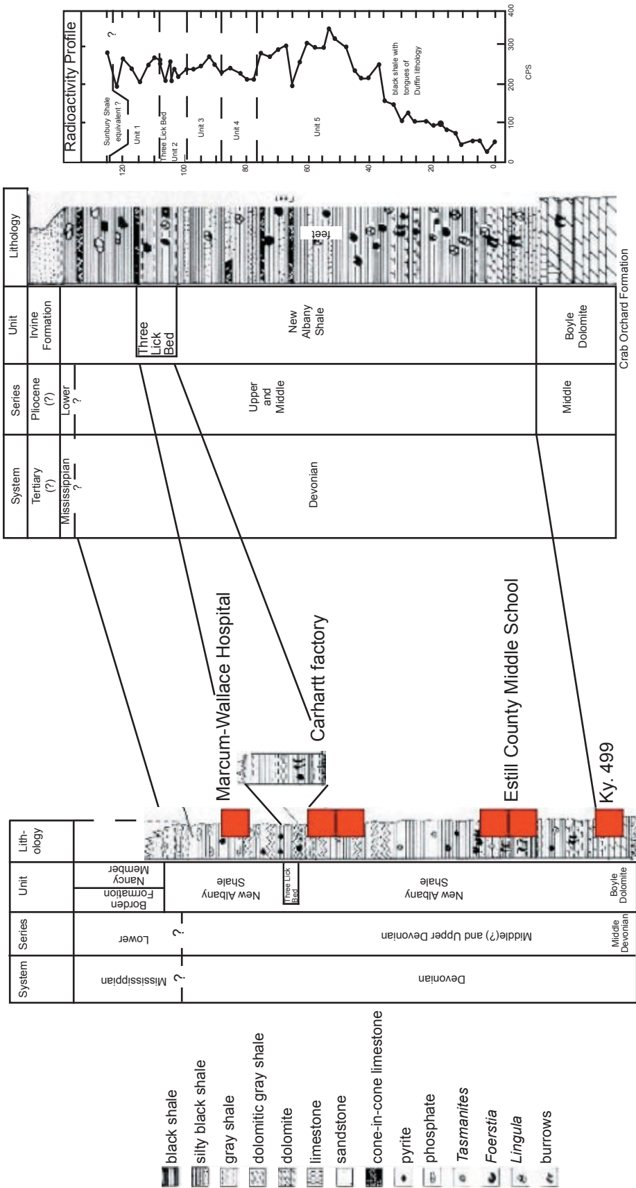
Figure 12. Stratigraphic column showing location of buildings examined in this study. Stratigraphic columns modified from Swager (1978).
