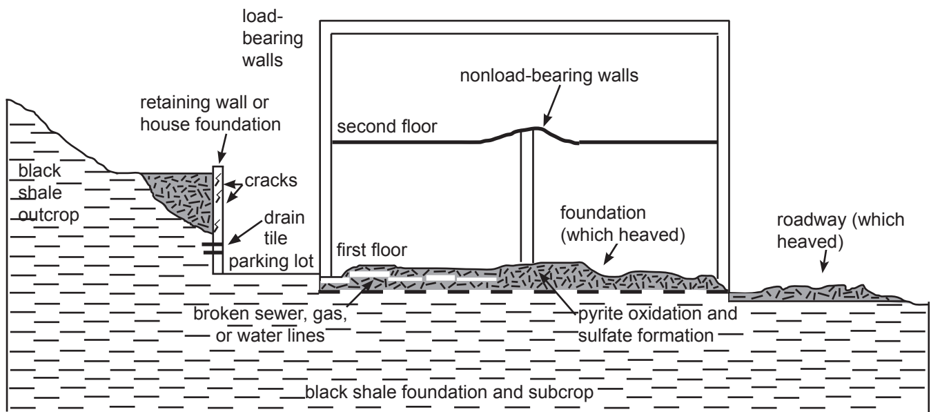
Figure 26. Schematic diagram of Chattanooga Shale outcrop, demonstrating pyrite oxidation and sulfate formation. Floors heave because sulfate forms and puts pressure on load-bearing walls. Roads, nonload-bearing walls, and retaining walls could be affected by continued pyrite oxidation and sulfate formation.
