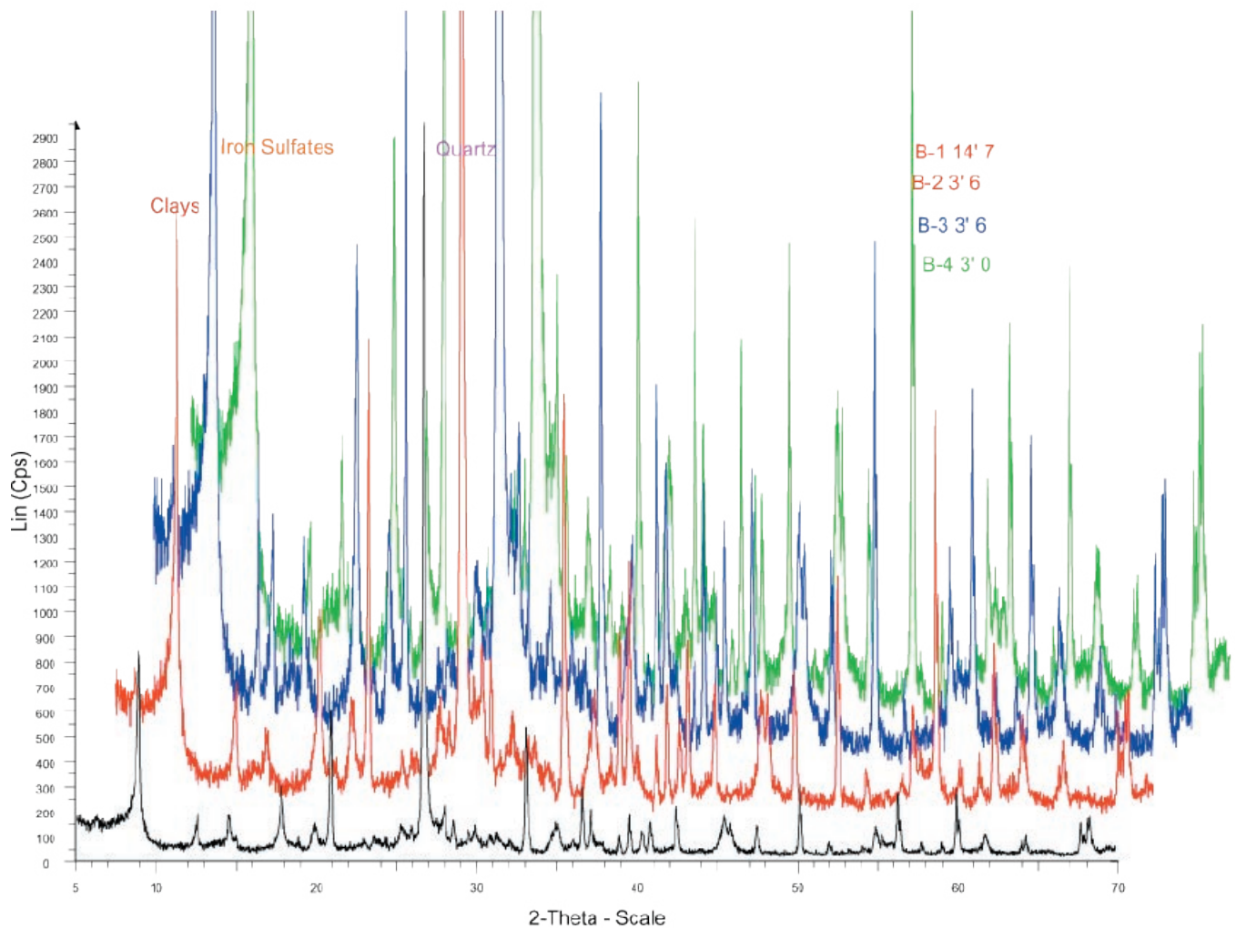
Figure 29. Diffractograms of cores in the study area show regions of clay minerals and sulfate activity between 10-20 2-theta. Data is projected in a three-dimensional view.
