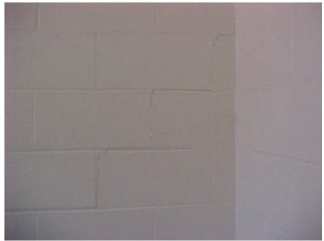
Figure 28. Cracks in concrete blocks at hospital.
