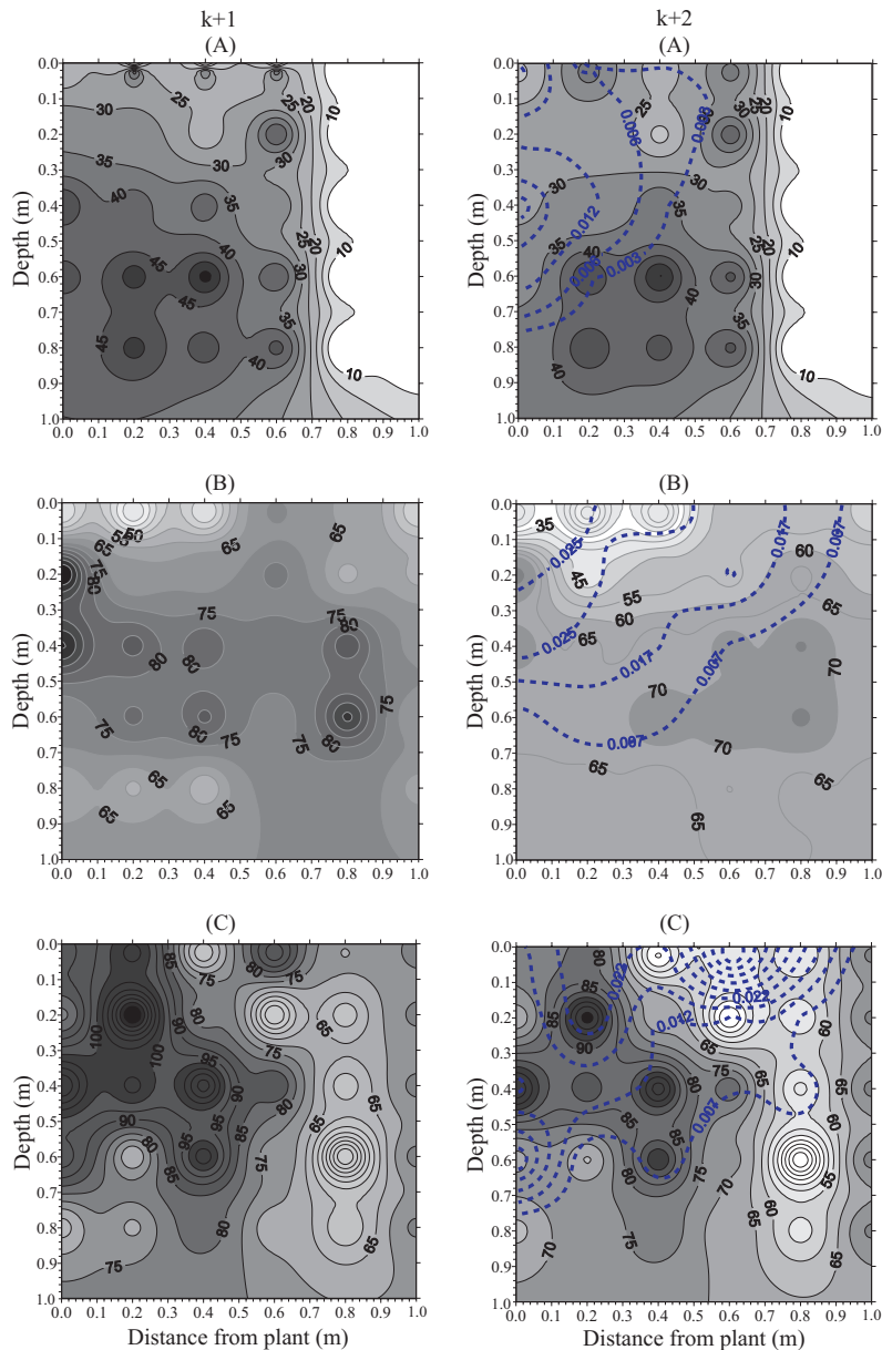
Figure 2. Available water (%) in the soil profile at k+1 (water content got the maximum value at shallow locations and the wetting front reached the depth of 0.9 m) and k+2 (time of the next irrigation) times for treatments T1 (A, two 4-L h -1 emitters per plant), T2 (B, four 4-L h -1 emitters per plant) e T3 (C, five 4-L h -1 emitters per plant). Dashed lines at time (k+2) indicate zones of water extraction.
