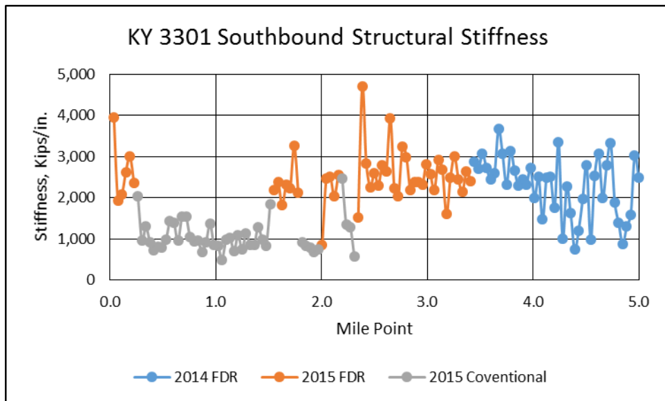
Figure D5. KY 3301 Southbound Structural Stiffness.
