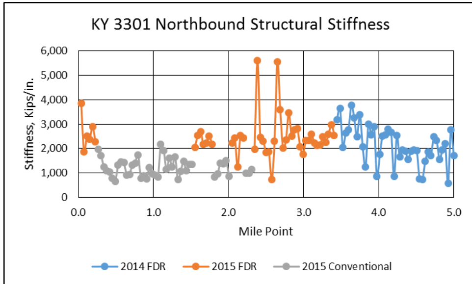
Figure D4. KY 3301 Northbound Structural Stiffness
