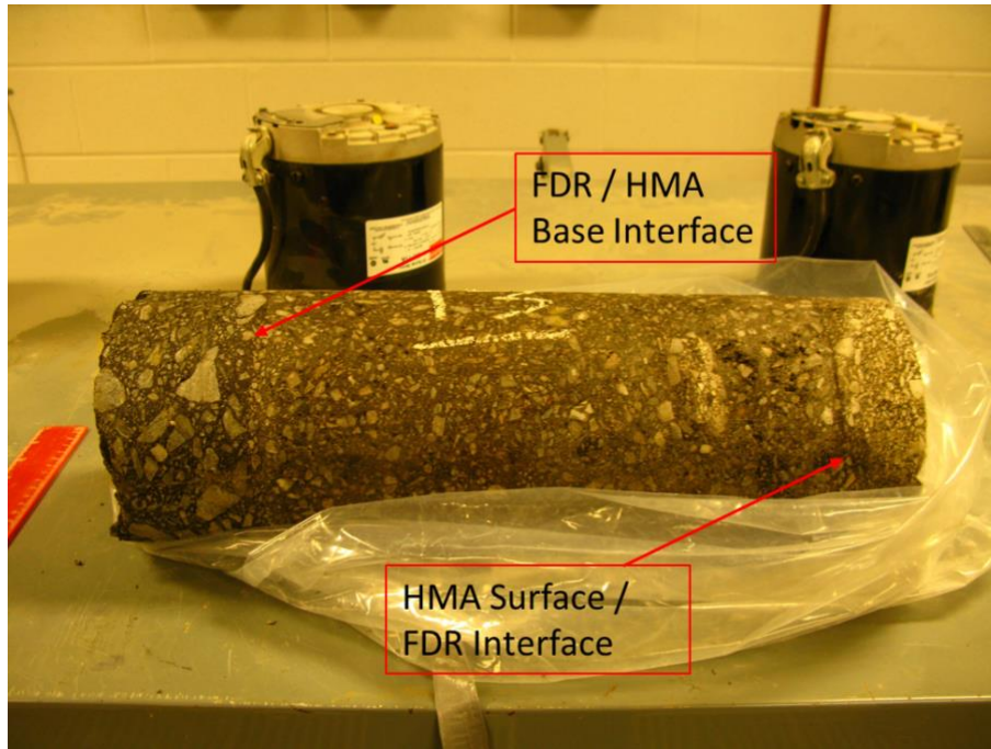
Figure E1. Full Depth Reclamation sample # 13 prior to trimming for compressive strength testing shows unreclaimed HMA material below the reclaimed materials.
