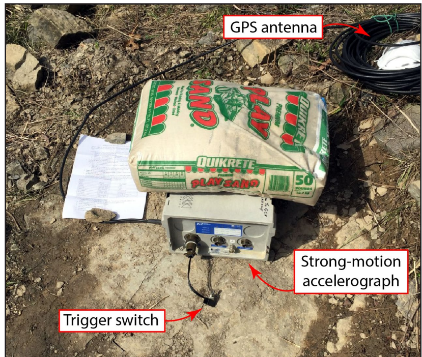
Figure 2. Instrumentation at station CPT3. Photo by Zhenming Wang.
