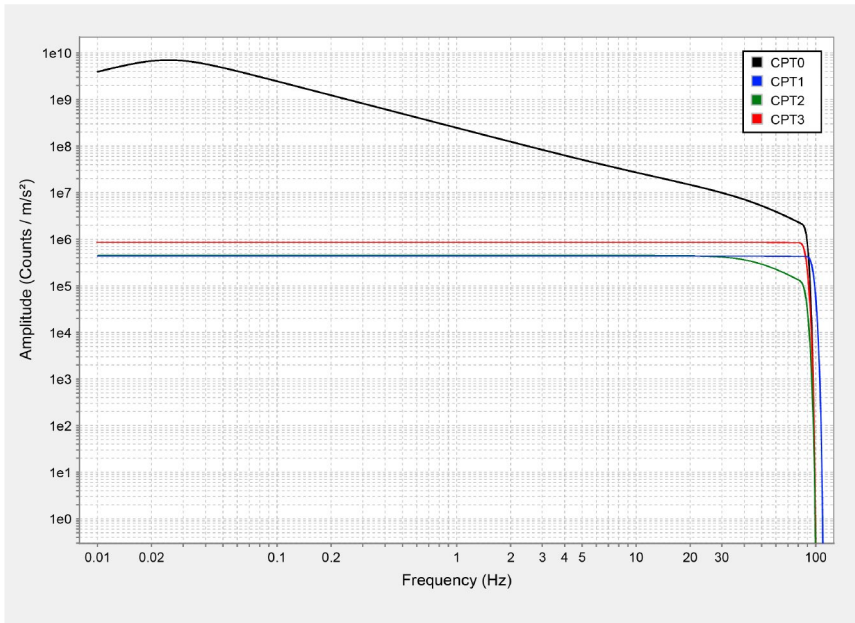
Figure 3. Amplitude responses from input ground acceleration for the instruments used at each site. Differences between the responses of each orthogonal component for a particular instrument are indistinguishable on this plot, and only the vertical-component frequency responses are shown.
