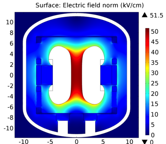
FIG. 9. Result of a finite element electrostatic calculation, performed using COMSOL, 33 of the Rogowski electrodes mounted inside the CV. For this calculation, the gap between the two electrodes was set to 2 cm and the two electrodes were held at +50 kV and -50 kV.
