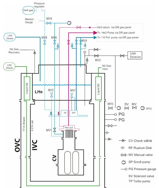
FIG. 3. MSHV plumbing diagram.
