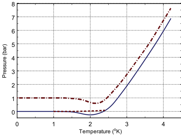
FIG. 14. Pressure of confined liquid helium plotted as a function of the temperature. Solid and dashed lines : the cell sealed at 1 K at the saturated vapor pressure (see text for details). Dotted-dashed line : the cell sealed at 1 K at a pressure of 1 bar.
