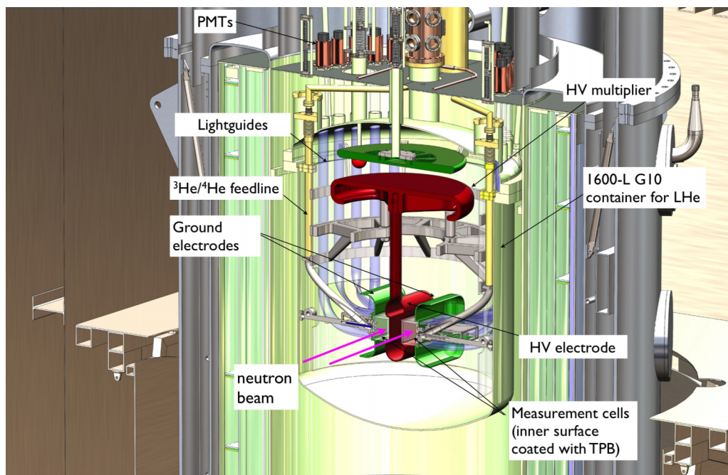
FIG. 1. A schematic of the central part of the SNS nEDM experiment, as it is currently designed.
