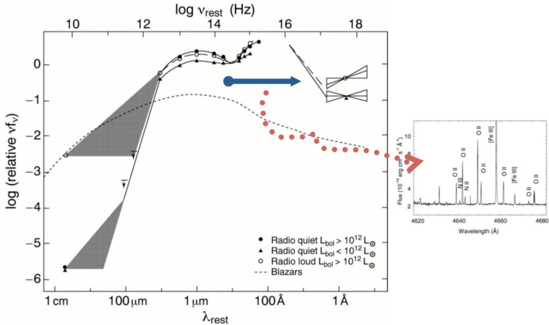
Fig. 2. The “primary mechanism”, converting an SED into emission lines. The color figure can be viewed online.
