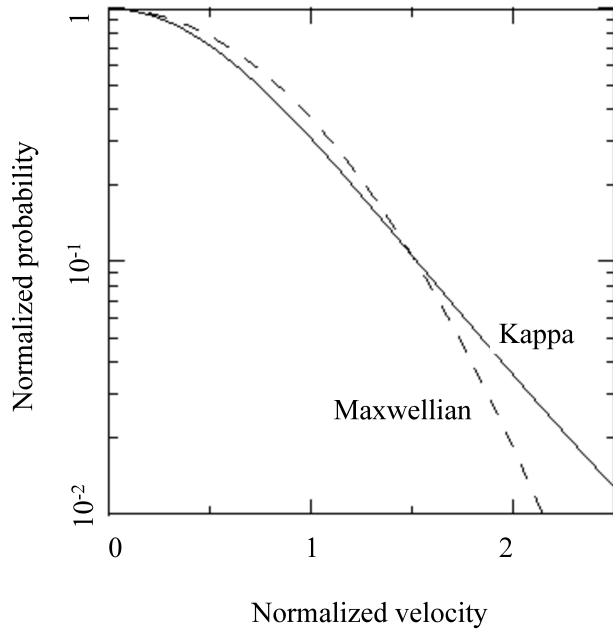
Fig. 1. Comparing a Maxwellian with a kappa electron velocity distribution. The kappa distribution has more high-energy electrons than a thermal gas. Smaller values of kappa correspond to greater deviations from a Maxwellian while a thermal distribution has a kappa of infinity. Equation 1 shows the relation between t^2 and kappa.
