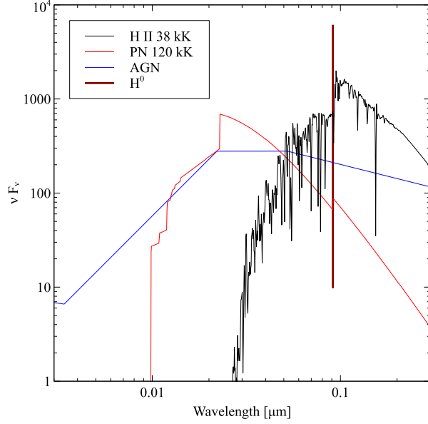
Fig. 3. The SEDs of an O star, a PN central star, and a typical AGN, as shown. The vertical line indicates the ionization potential of hydrogen. The color figure can be viewed online.
