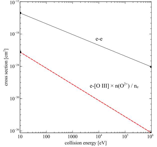
Fig. 4. Comparison of the e-e collision cross section with the cross section for exciting the O III green line. The color figure can be viewed online.
