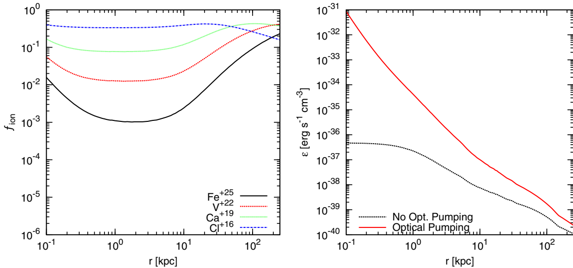
Figure 10. Virgo cluster results: Left panel: Ionization fractions for several hydrogenic ions with Z \geq 17 . The fractions are constant within the central 2 kpc in the absence of the Virgo A radiation. Right panel: impact of the AGN radiation field on the emissivity of the ^{57}\text{Fe XXVI } \lambda 348 \mu\text{m} line. Even though the AGN is not as bright as Perseus A, the emissivity boost is at least one order of magnitude within the central 10 kpc.
