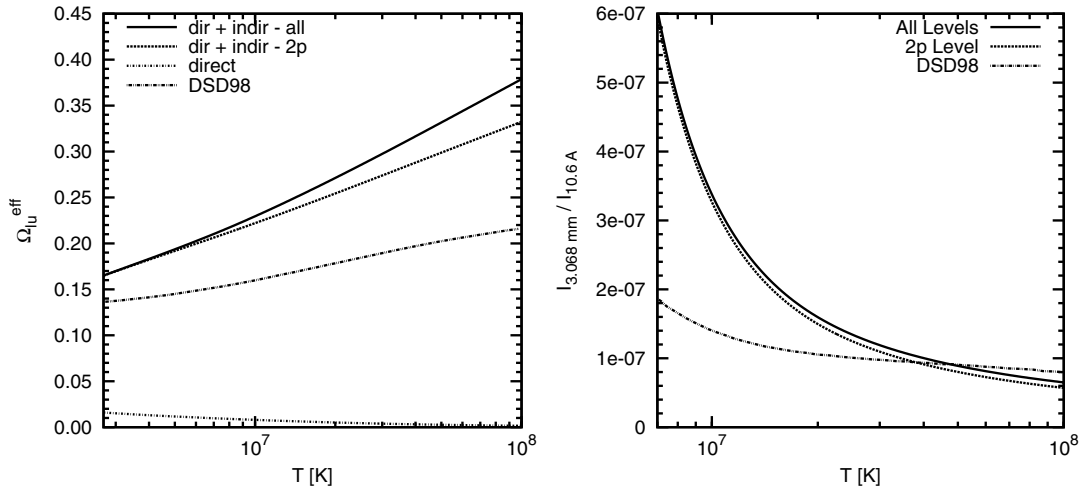
Figure 1. Left panel: effective collision strength as a function of temperature. Right panel: hyperfine line intensity in units of the 10.6 Å X-ray doublet. In both plots, the excitations shown are direct (dot–dashed), indirect through the 2 p level (dashed), and through all higher levels in CLOUDY (solid). The results of D’Cruz et al. (1998) are also shown (dot–dot–dashed).
