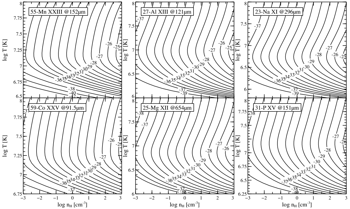
Figure 4. Log intensity maps for the coronal hyperfine lines in order of descending peak intensity from left to right, and from top to bottom. (The complete figure set (14 images) is available in the online journal.)
