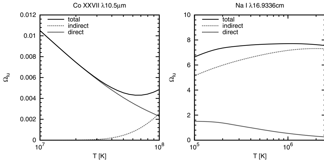
Figure 2. Collision strength decomposition for hydrogenic cobalt (left panel) and neutral sodium (right panel). The dominant mode of collisional excitation depends on the iso-sequence.
