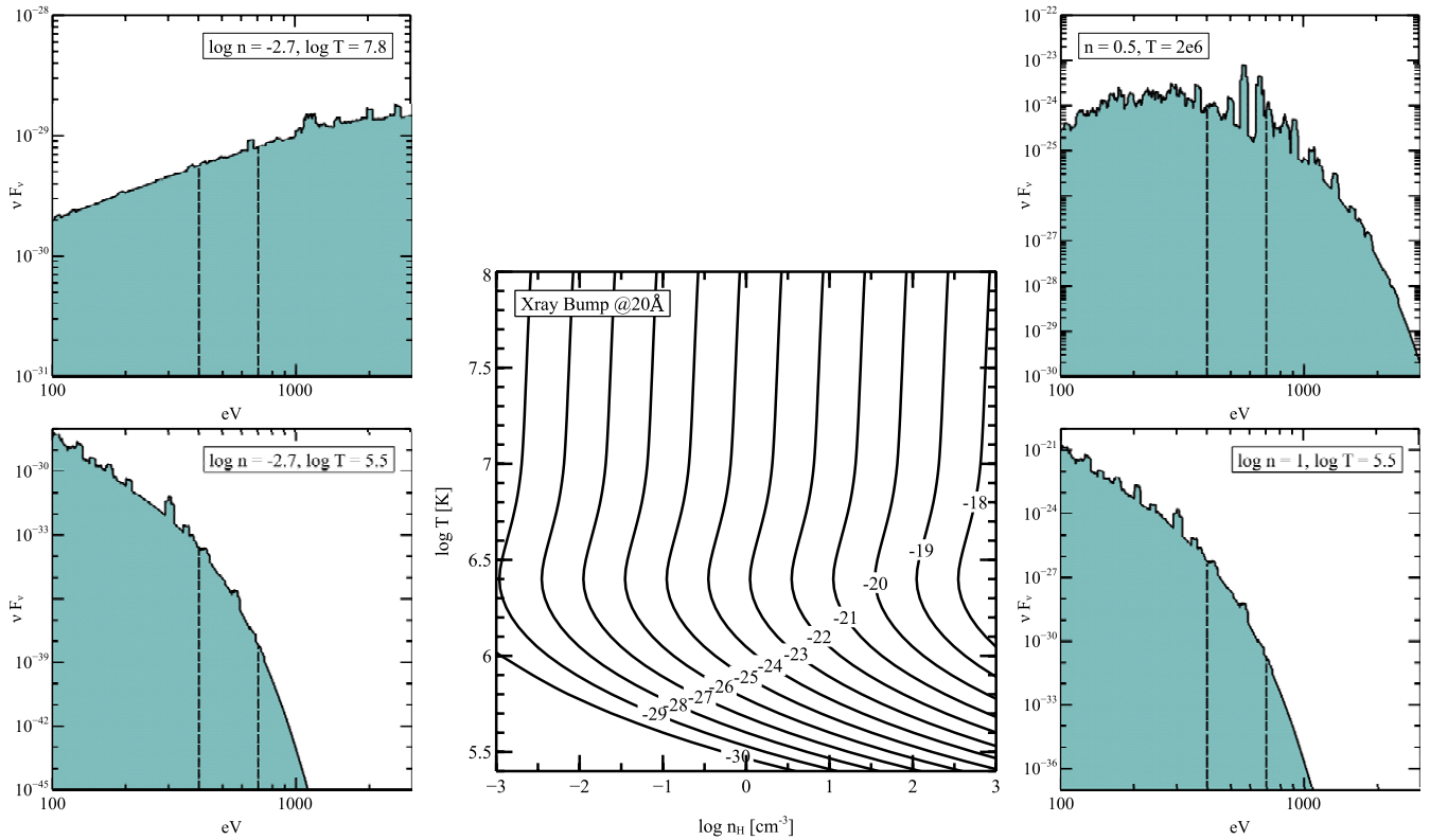
Figure 5. Center: Intensity contours of the X-ray complex at 20 Å (see the text), including the bremsstrahlung continuum. Left and right: X-ray spectra in the range 0.1–3 keV for various points in the grid, as indicated in the legends. The density and temperature for the top right spectrum are similar to the conditions of the hot gas in the Extended Orion Nebula (Güdel et al. 2008). The spectra are at higher resolution than typically attainable in X-ray observations.
