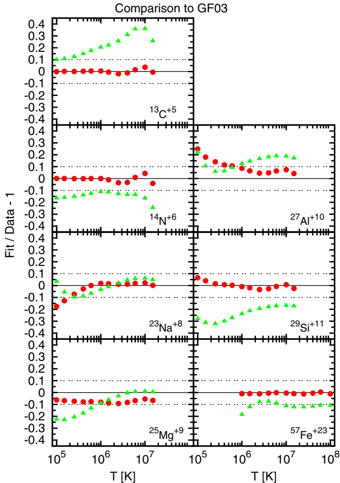
Figure 12. Comparison of the fit residuals to the total effective collision strength of the ZS00 data for the present work (red solid circles) and the work of GF03 (green solid triangles). The dashed lines indicate \pm 10\% deviations from the data.
