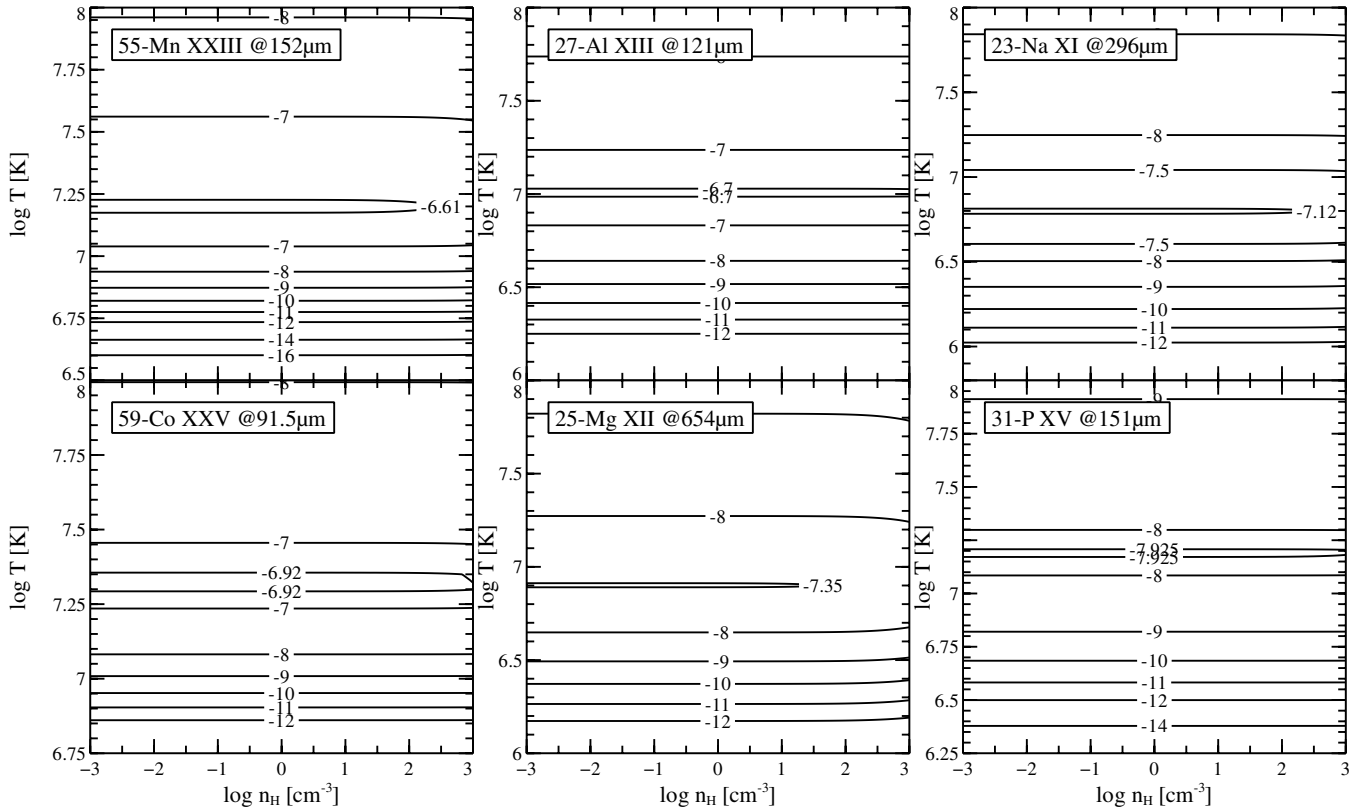
Figure 6. Intensity maps for the coronal hyperfine lines normalized by the intensity of the X-ray line complex. The images are presented in the same order as Figure 4. (The complete figure set (11 images) is available in the online journal.)
