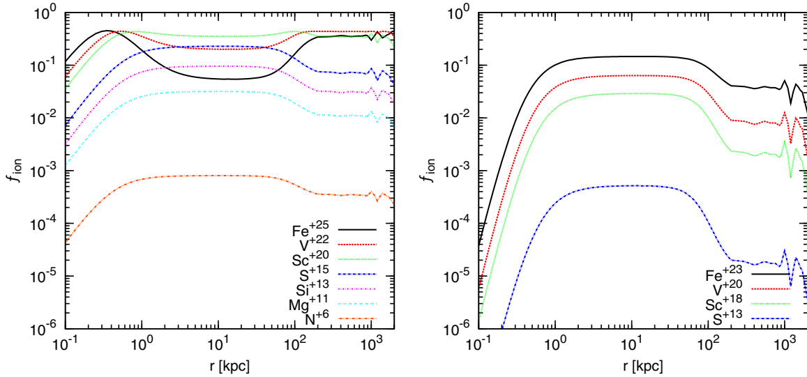
Figure 7. Example ionization fraction profiles for hydrogenic (left panel) and lithium-like (right panel) ions. The effects of the AGN radiation are prominent within the central 2 kpc. Note that the temperature profile rises beyond 100 kpc from a central floor of about 3 keV to about 6.5 keV at 900 kpc. The structure seen around 1 Mpc is due to uncertainties in the input ROSAT temperature profile.
