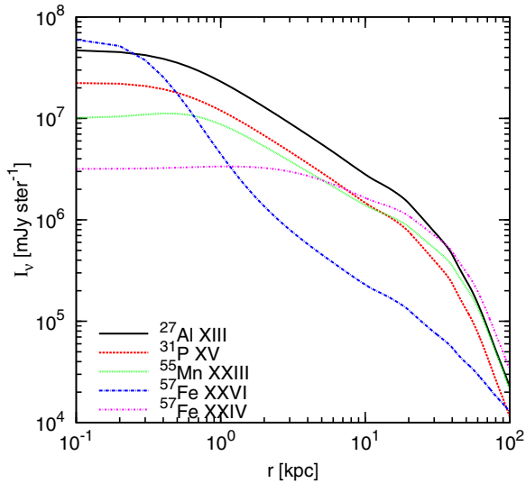
Figure 9. Intensity profiles within (projected) 100 kpc of NGC 1275 for the five brightest hyperfine lines.
