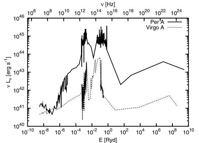
Figure 13. Spectral energy distribution of NGC 1275 and 3C 274. See the text for details.
