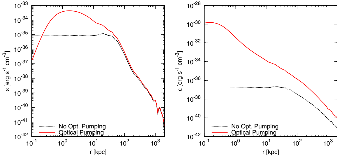
Figure 8. Comparison of the predicted emissivity profile of the ^{57}\text{Fe} xxiv \lambda 3.068 mm (left panel), and the ^{57}\text{Fe} xxiv \lambda 348 \mu\text{m} (right panel) lines in Perseus, with the effects of optical pumping accounted for and ignored.
