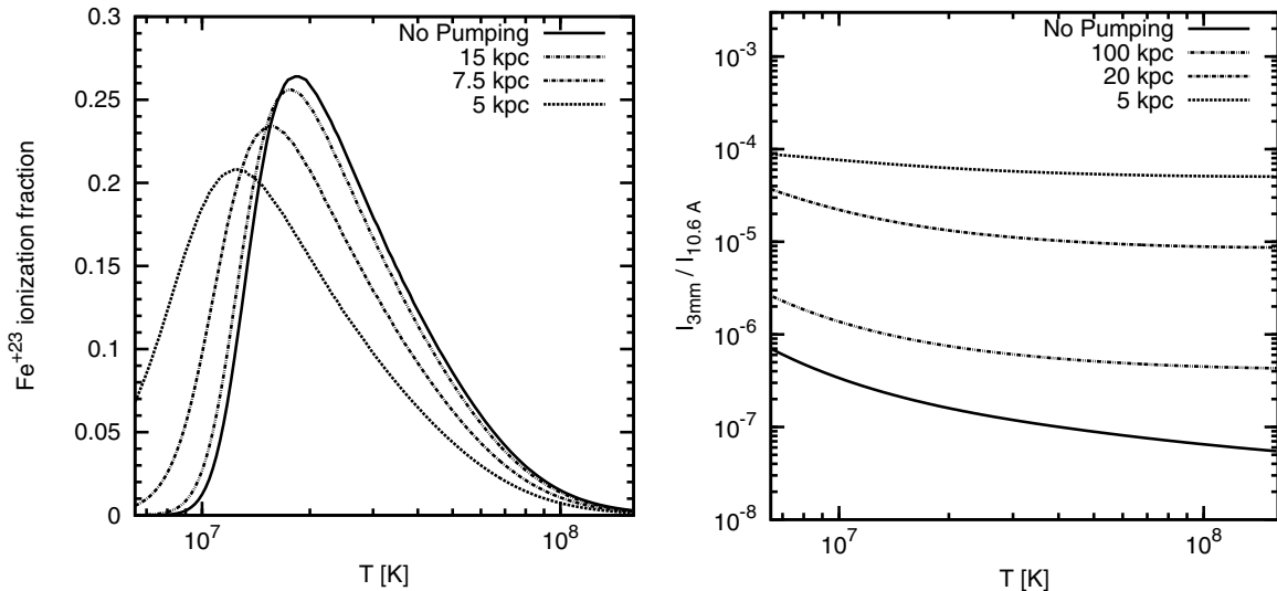
Figure 3. Temperature variation of (left panel) the ionization fraction of \text{Fe}^{+23} and (right panel) the ratio of the hyperfine line over the 10.6 \text{ \AA} X-ray doublet, as a function of point source proximity. Solid lines illustrate purely collisional results, while other line types represent results at various central distances, as indicated in the keys.
