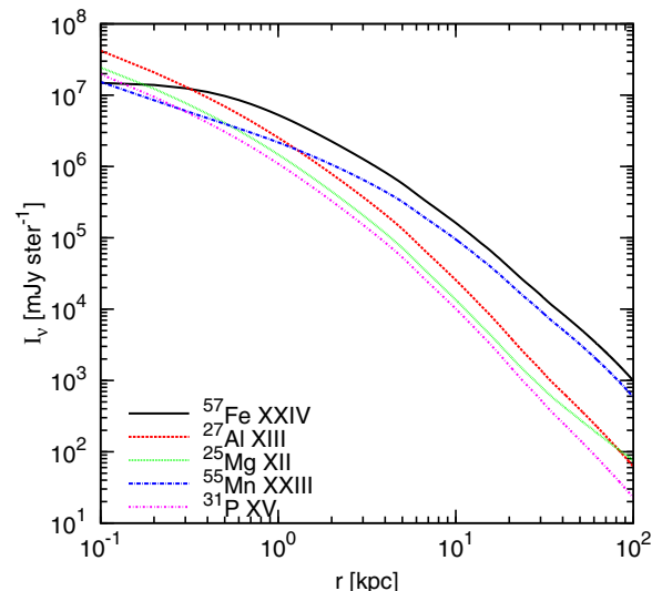
Figure 11. Intensity profiles for the five brightest lines in the Virgo cluster. (A color version of this figure is available in the online journal.)
