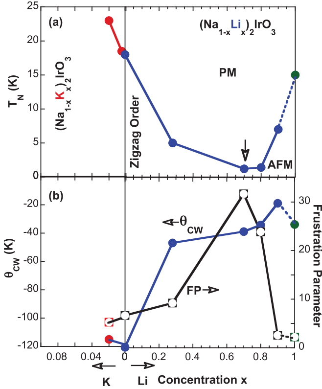
FIG. 3. (Color online) Ordering and interaction scales of (\text{Na}_{1-x}\text{A}_x)_2\text{IrO}_3 ( A = \text{Li} or \text{K} ) as a function of x . (a) The Néel temperature T_N , and (b) the Curie-Weiss temperature \theta_{\text{CW}} (left scale) and the frustration parameter (right scale) as a function of x . Note that K doping increases T_N , in sharp contrast to Li doping, and that the green data points for \text{Li}_2\text{IrO}_3 ( x = 1.0 ) are obtained from Ref. [10].
