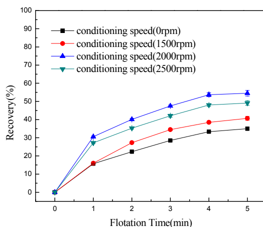
Figure 6. Effect of conditioning speed under natural atmosphere on the recovery of mixed minerals, with pyrrhotite and chlorite mixed at a ratio of 10:1 (pH = 9.0 \pm 0.2 ; C(potassium amyl xanthate) = 1 \times 10^{-4} mol/L; C(MIBC) = 1 \times 10^{-4} mol/L; and Conditioning time = 5 min).
