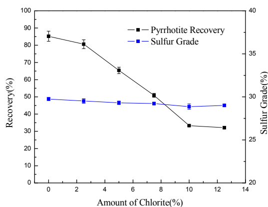
Figure 3. Effect of chlorite on the flotation recovery of pyrrhotite and grade of sulfide (pH = 9.0 ± 0.2; C(potassium amyloxanthate) = 1 × 10 -4 mol/L; C(methyl isobutyl carbinol (MIBC)) = 1 × 10 -4 mol/L).
