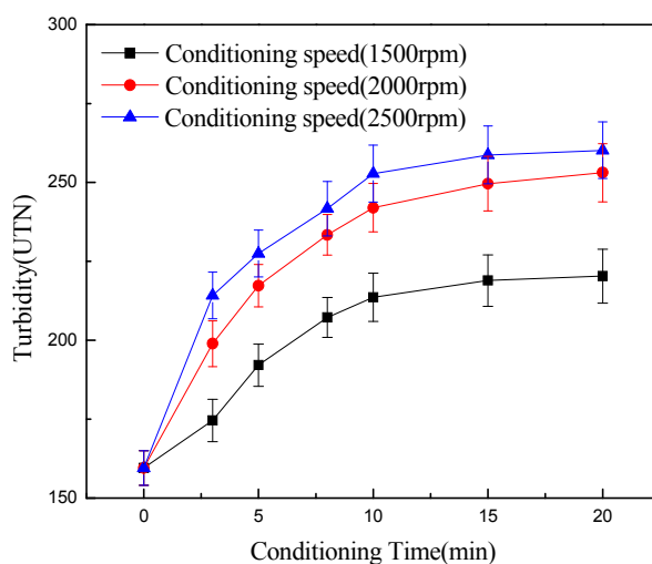
Figure 5. Turbidity of mixed minerals (pyrrhotite and chlorite were mixed by 10:1) as a function of conditioning speed and time of pH = 9.0 ± 0.2.
