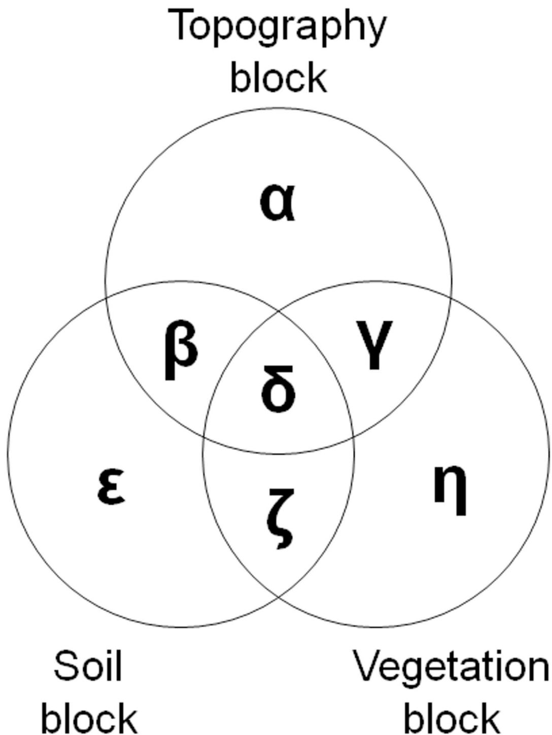
Fig 2. Representation of bi-variance ( \beta+\gamma+\delta+\zeta , all in %) and tri-variance ( \delta , in %) in vegetation–soil–topography relationships. Symbols, \alpha , \epsilon , and \eta , represent uni-variances. The three circles here are of the same size because the corresponding three singular axes have been standardized (see text).
