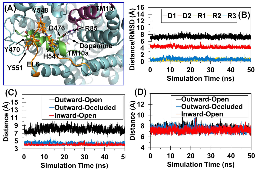
Figure 2. MD-simulated WT hDAT structures in the three typical conformational states. (A) Structural model of WT hDAT in the outward-occluded state. hDAT is in cyan cartoon style. TM1b (the second part of transmembrane helix 1), TM10a, and EL6 are in purple, green, and orange, respectively. Dopamine and key residues are shown in stick-ball style. Hydrogen bonds between D476 and R85 are indicated in dashed lines. (B) Tracked distances and positional RMSD values for WT hDAT. D1 indicates the tracked internuclear distance between the C \alpha atoms of Y470 and Y548. D2 refers to the tracked internuclear distance between C \gamma atom of D476 and the C \zeta atom of R85. The tracked changes of the RMSD for the C \alpha atoms of Y470, R85, and D476 are indicated by R1, R2, and R3, respectively. (C) Tracked internuclear distance between the C \gamma atom of D476 and the C \zeta atom of R85 in three typical conformational states of WT hDAT. (D) Tracked internuclear distance between the C \alpha atoms of Y470 and Y548 in three typical conformational states of WT hDAT.
