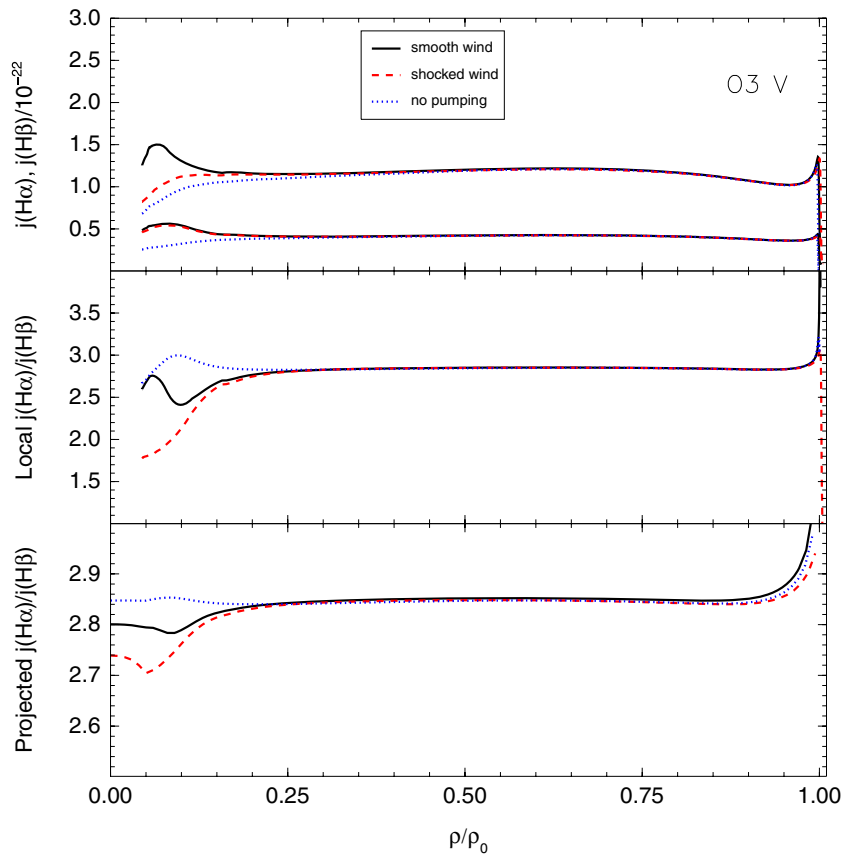
Figure 11. As in Figure 10, for the case of an O3 V star. (A color version of this figure is available in the online journal.)
