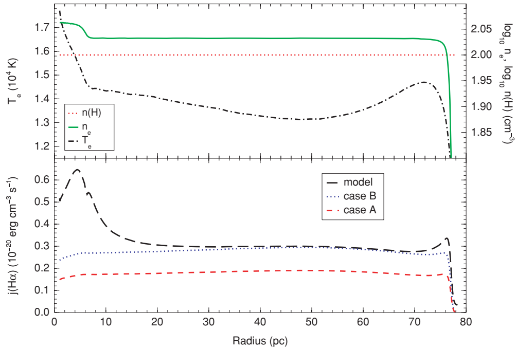
Figure 2. Upper panel: physical conditions in a model low-metallicity giant H II region ionized by a 3 Myr stellar population (see Section 2 for details). Lower panel: normalized H \alpha emissivity profile of the model, compared with case A and B predictions.
