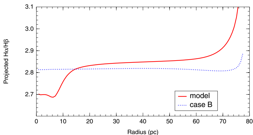
Figure 6. Solid line: H\alpha/H\beta projected profile along the nebular midplane. Dotted line: H\alpha/H\beta projected profile computed assuming case B emission. (A color version of this figure is available in the online journal.)
