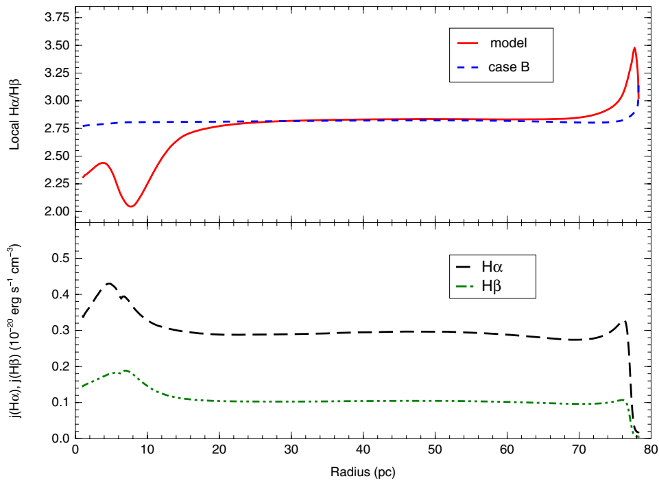
Figure 5. Top panel: local H\alpha/H\beta intensity ratio as a function of radius in model M2, compared with the case B value at the model’s local temperature. Bottom panel: normalized H\alpha and H\beta emissivity profiles.
