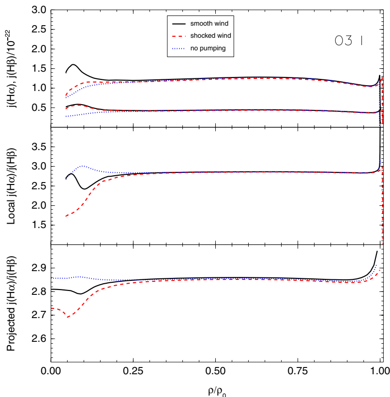
Figure 10. Local emissivities, local Balmer line ratios, and projected Balmer line ratios of photoionization models illuminated by WM-basic models of an O3 I star, with a smooth wind-velocity law (solid) and a shocked wind (dashed), compared with those of a model with no fluorescent excitation (dotted). Emissivities are in units of \text{erg s}^{-1} \text{cm}^{-2} . The distances to the stars are normalized to the maximum nebular radius in each case.
