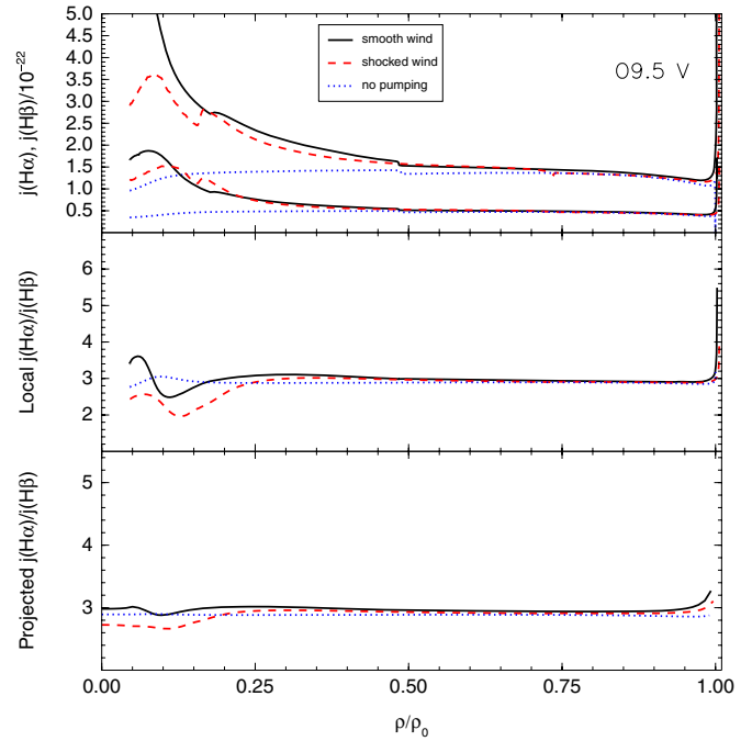
Figure 13. As in Figure 10, for the case of an O9.5 V star. (A color version of this figure is available in the online journal.)
