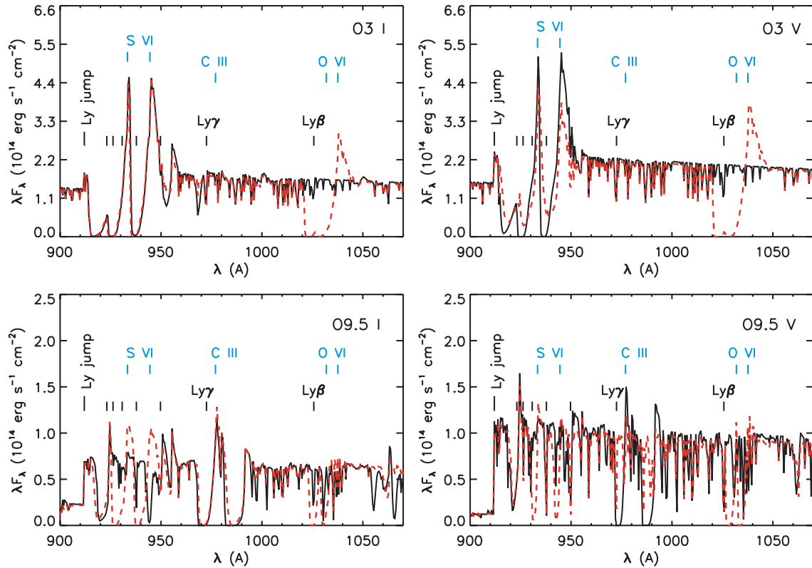
Figure 9. WM-basic models for stars of different spectral types and luminosity classes (see Table 8 for the main models' properties). Black solid lines: models with a smooth wind-velocity law; light dashed lines: shocked-wind models. The main stellar spectral features that may affect case D predictions are indicated. (A color version of this figure is available in the online journal.)
