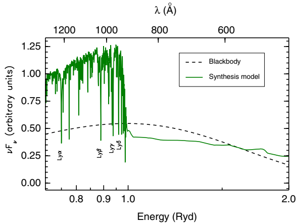
Figure 1. Comparison between the SEDs of a population synthesis model and a blackbody at T_{\text{eff}} = 40\text{k K} , normalized to the same number of ionizing photons. The position of the first four Lyman lines is also shown.
