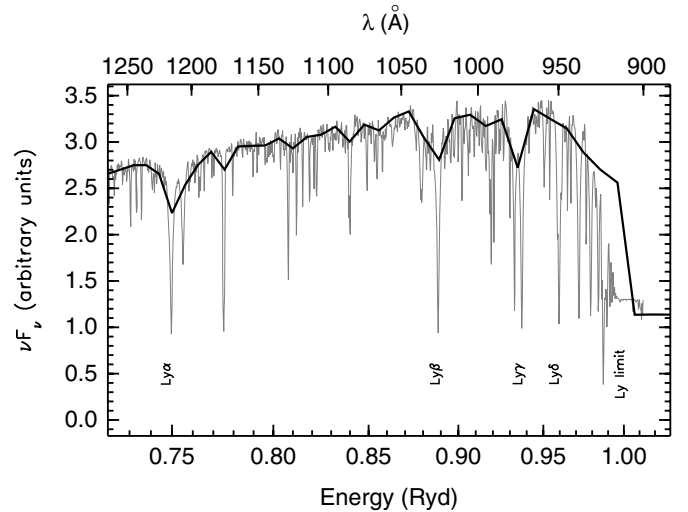
Figure 3. UV SED of a 3 Myr, Z = 0.001 stellar population, in low resolution (thick black line, spectral sampling = 10 Å) and high resolution (thin gray line, spectral sampling = 0.3 Å). Also shown are the first four Lyman lines, from Ly \alpha at \lambda = 1215 Å (which does not produce any Balmer photon) through Ly \delta at 950 Å.
