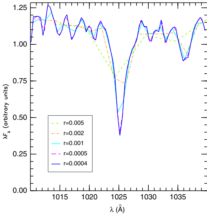
Figure 4. HR synthesis model rebinned by Cloudy to different values of the spectral resolution r = \Delta\lambda/\lambda .
