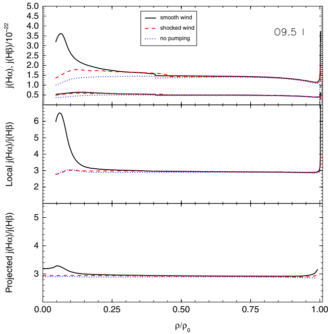
Figure 12. As in Figure 10, for the case of an O9.5 I star. (A color version of this figure is available in the online journal.)
