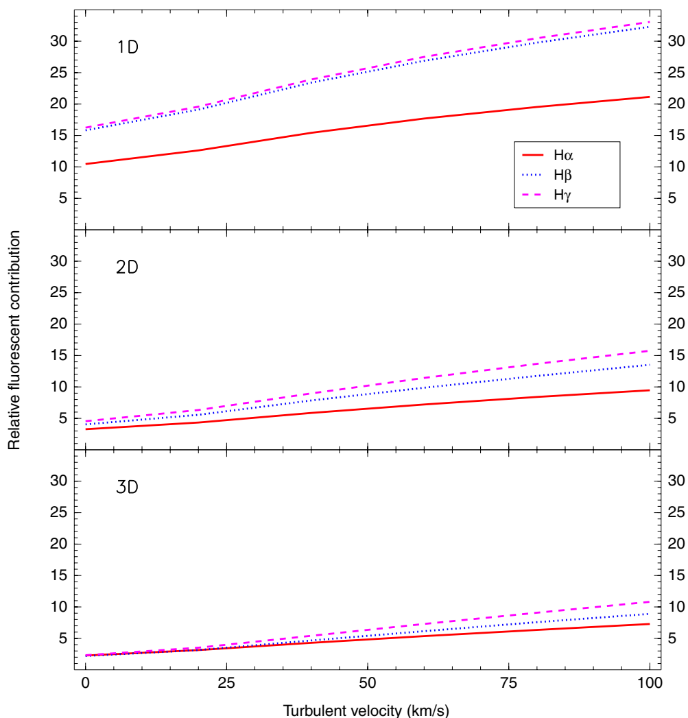
Figure 8. Relative contribution of fluorescent excitation to the intensities in H \alpha , H \beta , and H \gamma as a function of microturbulent velocity. (A color version of this figure is available in the online journal.)
