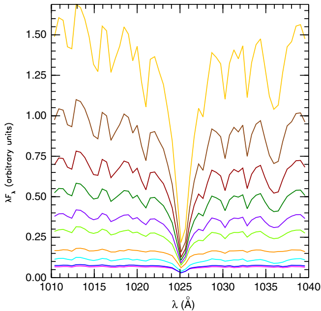
Figure 7. SEDs around Ly \beta of a sequence of synthesis models with increasing ages, normalized to the number of ionizing photons. From the bottom up: 2, 1, 3, 4, 5, 6, 7, 8, 9, and 10 Myr.
