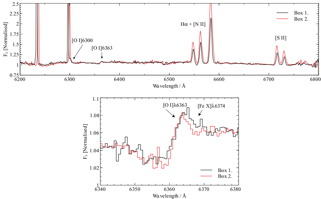
Figure 4. Top panel: spectra from box 1 (black) and box 2 (red) without continuum subtraction. All sky lines except [O I] \lambda 6300 and [O I] \lambda 6363 sky emission have been subtracted in order to more clearly see object emission-line features. Bottom panel: a blow-up of the expected [Fe x] \lambda 6374 region. Emission from cool gas in box 2 has a broader velocity width than box 1 in general, except over the [O I] \lambda 6363 and [Fe x] \lambda 6374 regions. This demonstrates the excess flux on the red-wing of oxygen emission in box 1. This cannot be accounted for by subtraction of a template from the object [O I] \lambda 6300 emission line.
