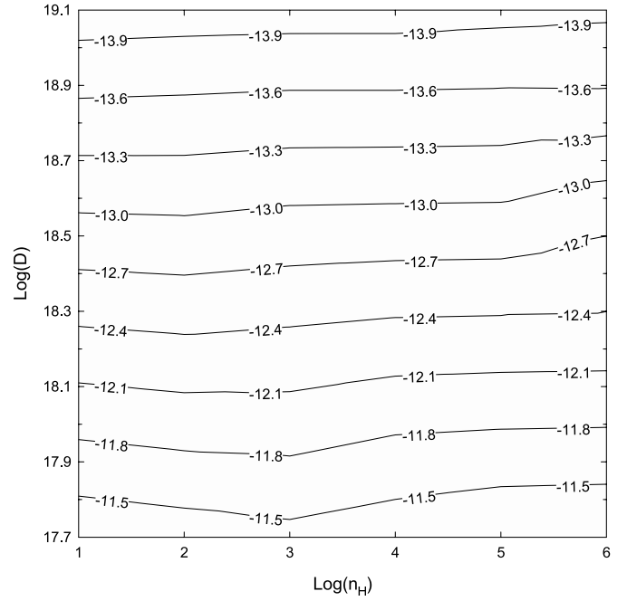
FIG. 7.—Log of the predicted H\beta surface brightness ( \text{ergs cm}^{-2} \text{ s}^{-1} \text{ arcsec}^{-2} ). The parallel horizontal contours are expected, given the inverse square relationship of surface brightness with distance. The actual surface brightness must be substantially smaller than the total observed surface brightness of 5 \times 10^{-12} ( \log [H\beta] = -11.3 ), which mainly comes from the main ionization front.
