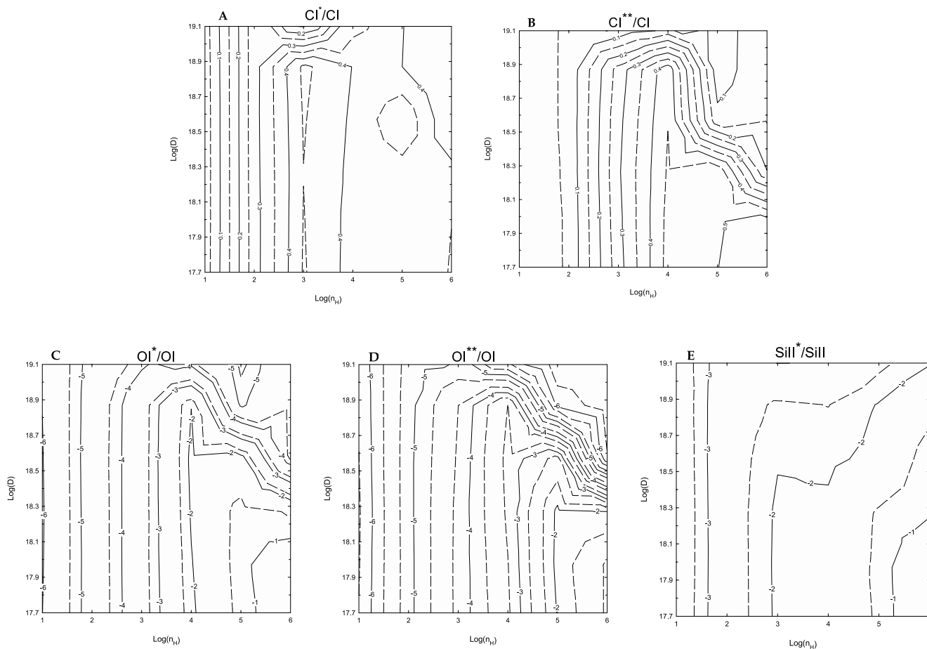
FIG. 4.—Ratio of the excited-state column densities of (a, b) C, (c, d) O, and (e) Si + relative to the ground state. The observed values, with 1 \sigma ranges when available, are N(\text{C I}^*)/N(\text{C I}) \sim -0.1 , N(\text{C I}^{**})/N(\text{C I}) \sim -0.2 , N(\text{O I}^*)/N(\text{O I}) \sim -3.5 \pm 0.7 , N(\text{O I}^{**})/N(\text{O I}) \sim -3.4 \pm 0.7 , and N(\text{Si II}^*)/N(\text{Si II}) \sim -1.4 \pm 0.4 . The parallel contours show their usefulness as density indicators.
