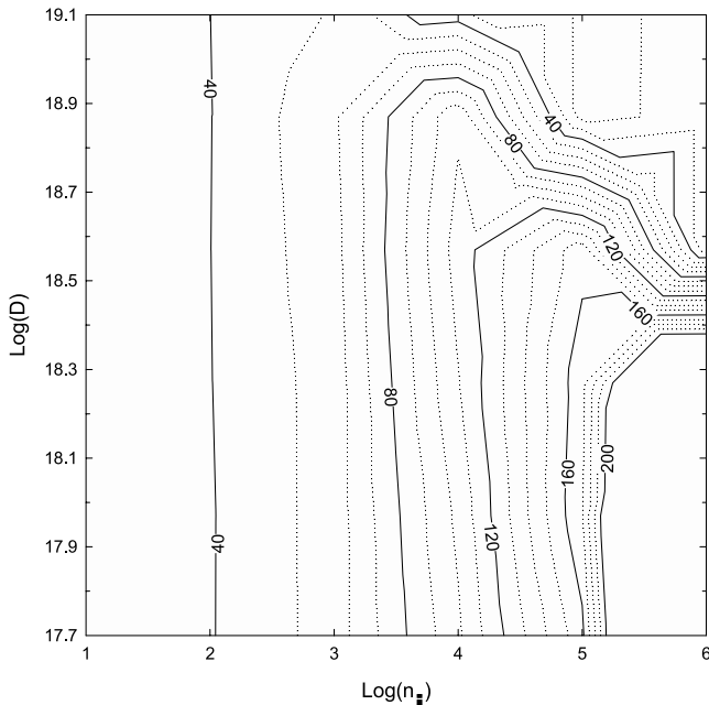
FIG. 6.—Predicted H\text{ I} spin temperature (K). For densities less than the critical density of [C\text{ II}] 158 \mu\text{m} ( 3 \times 10^3 \text{ cm}^{-3} ), the temperature remains relatively constant. However, for densities greater than this, [C\text{ II}] is no longer an efficient coolant, and the heating rate increases with a power of density greater than that for the cooling. The upper left corner corresponds to calculations that have a large abundance of molecules.
