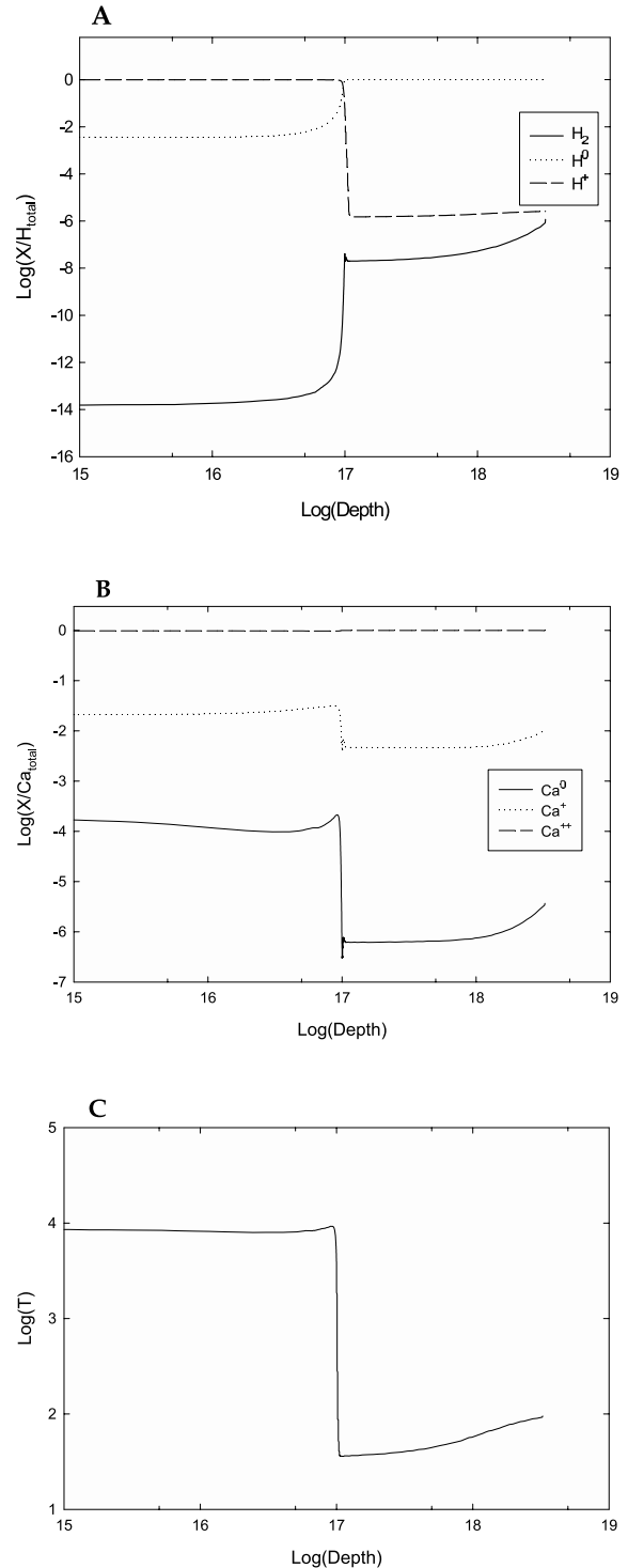
FIG. 10.—Fractional abundances of (a) H and (b) Ca in various forms as a function of depth (in cm) into the veil for our best model. Also shown is (c) the temperature vs. depth into the veil, with the temperature in kelvins. The drop in temperature corresponds to the hydrogen ionization front. Also of note is that our calculations predict the majority of calcium to be in the form of \text{Ca}^{++} .
