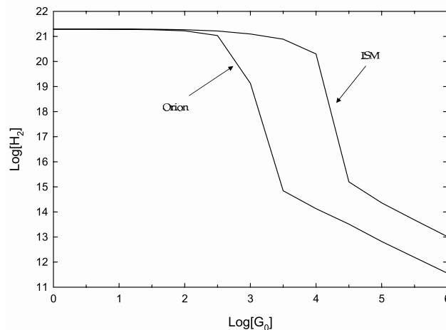
FIG. 12.—Column density of \text{H}_2 ( \text{cm}^{-2} ) for different grain-size distributions over a range of G_0 . For \log(G_0) < 2.5 , \text{H}_2 fully forms for both ISM and Orion grains. For larger values, the lack of small grains in the Orion distribution makes it less effective than ISM grains in shielding the \text{H}_2 dissociating continuum, and the dissociation rate becomes larger relative to the dissociation rate calculated using ISM grains. This process causes the two size distributions to differ by up to 6 orders of magnitude for some values of G_0 .
