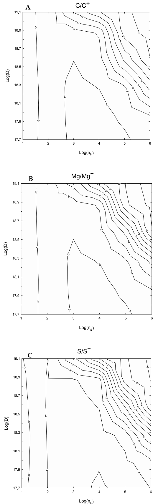
FIG. 3.—Log of the ratio of atomic to ionized (a) C, (b) Mg, and (c) S, which correspond to the column densities measured in more than one stage of ionization by SS97. The observed 1 \sigma ratios of C ( > -4.35 ), Mg ( -3.4 \pm 0.5 ), and S ( -4.2 \pm 1.0 ) agree with most of our calculations. In this and all subsequent contour plots, the parameter n_{\text{H}} = n(\text{H}^+) + n(\text{H}^0) + 2n(\text{H}_2) ( \text{cm}^{-3} ), the total hydrogen density in all forms.
