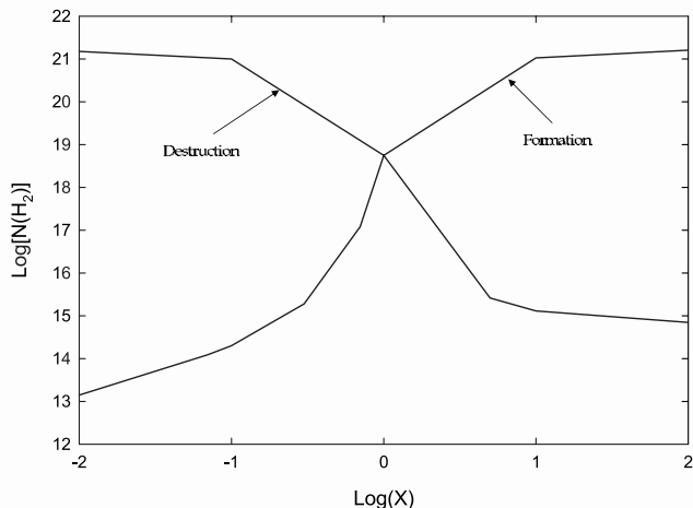
FIG. 11.—Predicted H 2 column density (cm -2 ) as a function of the dissociation and formation rate scaling factor X . This plot clearly illustrates the sensitivity of the H 2 column density to the various rates. Changes in either rate of an order of magnitude can cause changes to the H 2 column density of up to 6 orders of magnitude. In order to have confidence in predicting the H 2 column density, one must model the H 2 formation and destruction processes as accurately as possible, without resorting to approximations.
