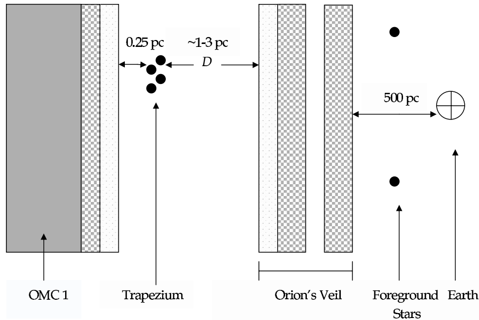
FIG. 2.—Geometry of the central regions of the Orion Nebula and the veil. For this figure, solid regions correspond to \text{H}_2 , checked regions to \text{H}^0 , and dotted regions to \text{H}^+ . Starting with the side of the veil facing the Trapezium, we have a small \text{H}^+ zone followed by a PDR. Because of the strong UV flux coming from the Trapezium cluster, \text{H}_2 never readily forms, but instead we have a thick region of atomic hydrogen. The segmented regions in the veil represent the multiple components seen in the 21 cm optical depth profile in Fig. 1. The distance D represents the distance from the side of the veil facing the Trapezium to the Trapezium itself and is the same distance used in all subsequent contour plots. [See the electronic edition of the Journal for a color version of this figure.]
