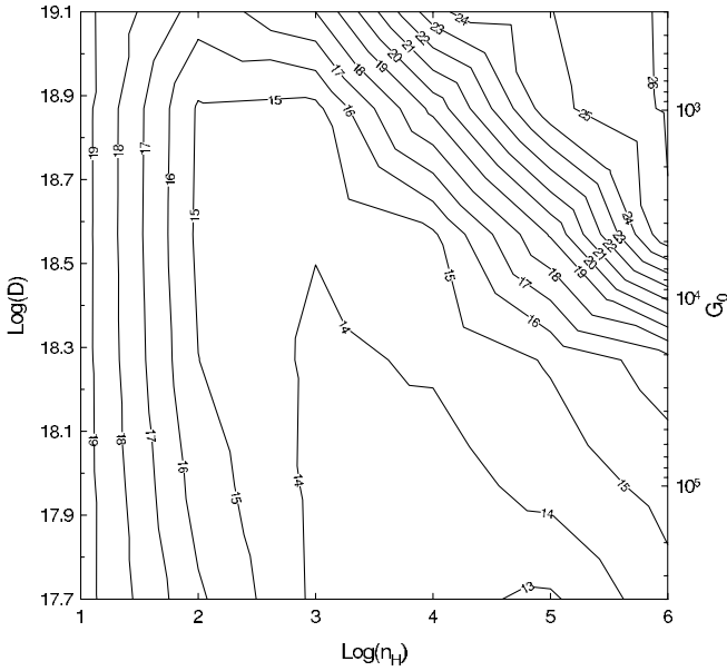
FIG. 5.—Log of the predicted H_2 column density ( \text{cm}^{-2} ). Copernicus observations set an upper limit of N(H_2) < 3.5 \times 10^{17} \text{ cm}^{-2} ( \log [N(H_2)] < 17.55 ). In addition to distance, on the right the scale is in units of the average UV radiation field (TH85). For the range of densities that our calculations predict for the veil ( 10^3 – 10^4 \text{ cm}^{-3} ), our calculations also predict an H_2 column density less than the Copernicus upper limit for distances less than \sim 10^{19.0} \text{ cm} . For very low densities, the large thickness of the H^+ region causes the value of G_0 to decrease because of geometrical dilution. By the time the hydrogen becomes atomic at these low densities, G_0 has decreased to 1 Habing for all distances. This is why the contours are vertical at low density.
