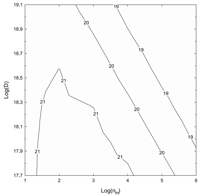
FIG. 9.—Log of the predicted \text{H}^+ column density ( \text{cm}^{-2} ). This is sensitive to the ionization parameter, which is the dimensionless ratio of flux to density. As expected, larger distances from the ionizing source (and hence smaller flux) and larger densities combine to lower the ionization parameter and hence the \text{H}^+ column density. For our best model, about 5% of the total hydrogen is in the form of \text{H}^+ .
