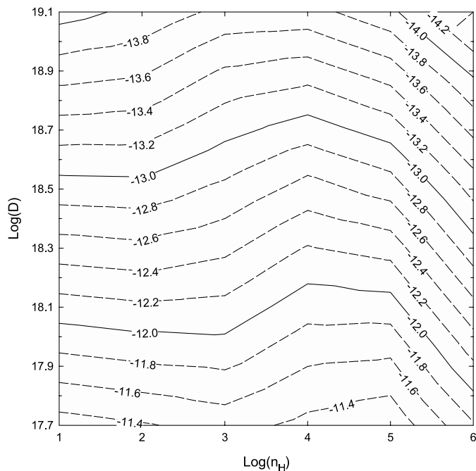
FIG. 8.—Predicted [N II] surface brightness ( \text{ergs cm}^{-2} \text{s}^{-1} \text{arcsec}^{-2} ). Based on calculations by O’Dell et al. (2003), the upper limit to the veil surface brightness is found to be 1.49 \times 10^{-13} \text{ ergs s}^{-1} \text{cm}^{-2} \text{arcsec}^{-2} ( -12.8 ). For the range of densities that our calculations predict are most likely for the veil ( 10^3 – 10^4 \text{ cm}^{-3} ), this corresponds to a lower limit to the distance of \sim 10^{18.5} \text{ cm} .
