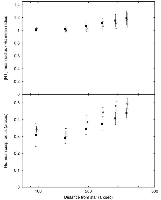
FIG. 13.—Model predictions for knot cusp radius as a function of distance from the central star. Bottom : Mean radius of \text{H}\alpha emission from the cusp in arcseconds. Top : Ratio of mean cusp radius in [\text{N II}] to that in \text{H}\alpha . Vertical bars indicate the range of values during the evolution of the models. Different symbol types correspond to models with differing treatment of the radiation hardening and photoelectric heating (see text).
