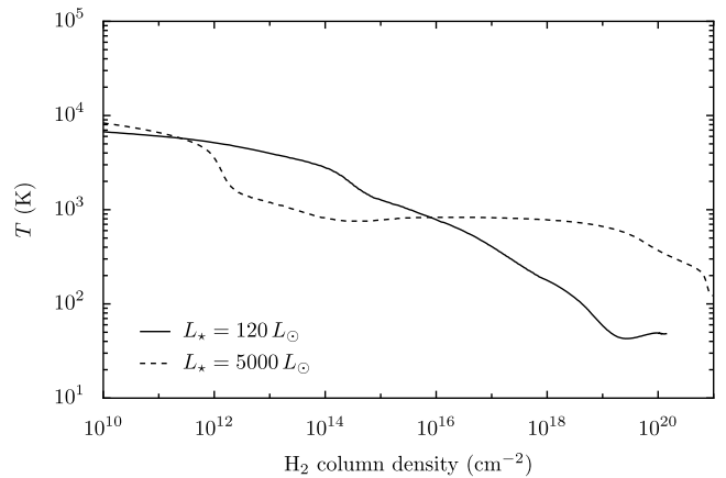
FIG. 15.—Gas temperature as a function of molecular hydrogen column density for our CLOUDY models of the knot PDR. The solid line shows a model calculated using our best estimates of parameters appropriate for the Helix knots. The dashed line shows the t = 4000 yr case considered by NH98. The largest difference is that the central star luminosity is about a factor of 40 larger. Grain photoelectric heating of neutral gas creates a significant warm (about 900 K) region.
