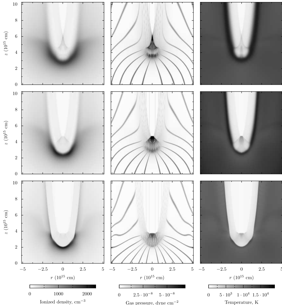
FIG. 12.—Physical structure of the model simulations at an age of 132 yr for a knot at a distance of 4.63 \times 10^{17} cm from the ionizing star. The three rows show simulations calculated using different degrees of hardening for the ionizing radiation (most hardening in the top row, no hardening in the bottom row). The three columns show ionized gas density, gas pressure, and gas temperature ( left to right ). The middle column also shows contours of the initial cylindrical radius of the gas at each point, which serve as approximate streamlines for the ionized part of the flow.
