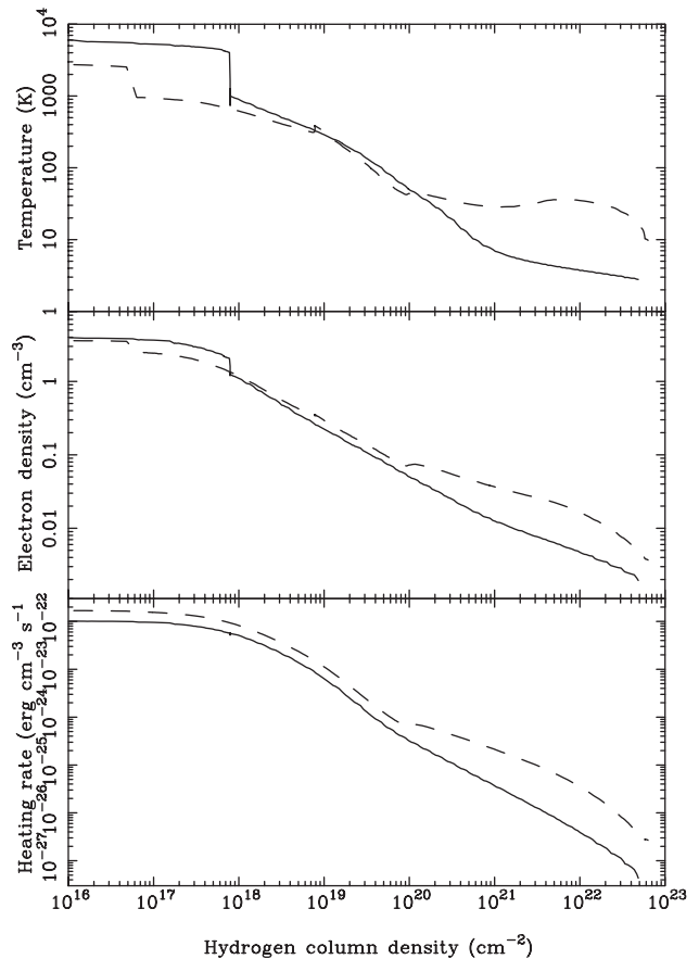
Figure 3. Comparison between CLOUDY version 84.09 (solid) and 90.04 (dashed). Note that these models are for the case of constant-density clouds (see Section 3 for the reason for this) and not the constant-pressure clouds computed by FFJ.
