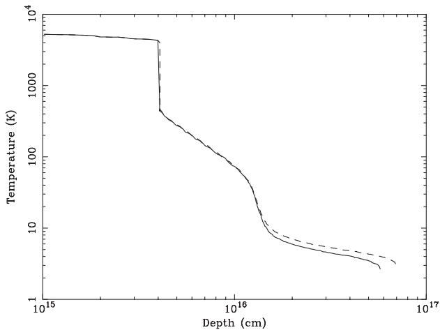
Figure 2. Temperature structure of the constant-pressure cloud, using the X-ray heating rates of Shull & van Steenberg (solid line) and Xu & McCray (dashed line), both in C84.09.
