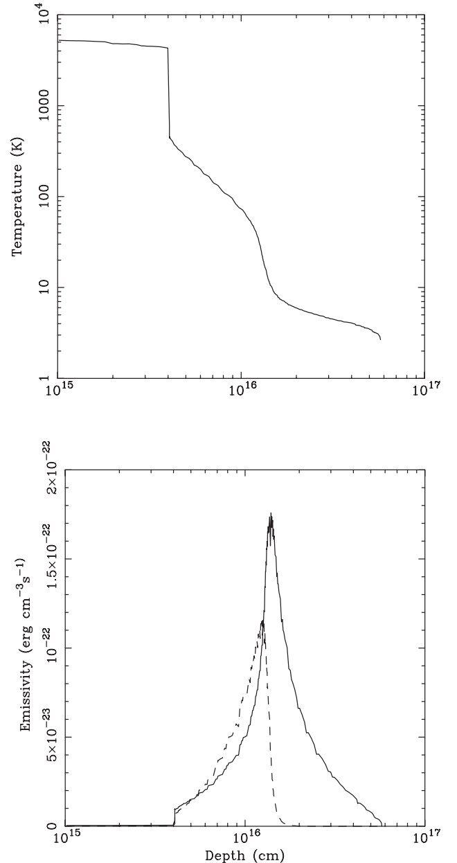
Figure 1. For the model computed in FFJ, using C84.09. (a) Upper panel: electron temperature as a function of depth into the cloud. (b) Lower panel: emissivity of [C I] 370 \mu\text{m} (dashed) and 610 \mu\text{m} (solid) lines as a function of depth into the cloud.
