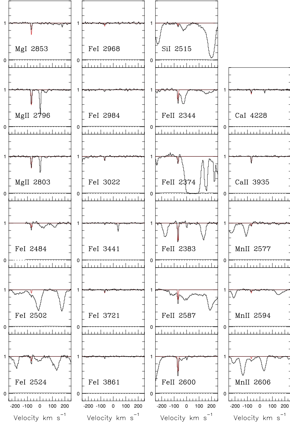
Figure 2. VLT spectrum (black) and photoionization model (red) in which Cloud 1 is modeled including unresolved saturation, and with \log Z = -1.0 , \log U = -8.2 , \log(N(\text{Mg II})) = 14.1 , and b = 0.2 \text{ km s}^{-1} .
