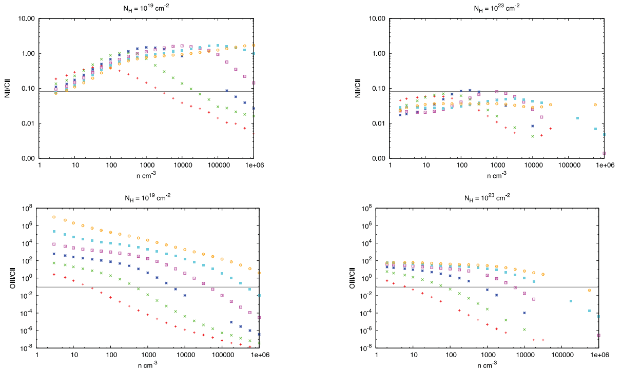
Figure 13. [N II]/[C II] (upper row) and [O III]/[C II] (lower row) versus density, n . Shown are the ratios for two different column densities, N_{\text{H}} = 10^{19} (left) and 10^{23} \text{ cm}^{-2} (right). [N II] and [O III] are produced in abundance at the surface of the cloud facing the ionization source and deplete with the depth of the cloud and, hence, sensitive probes of N_{\text{H}} . The different points have the same meaning as in Fig. 12. The horizontal lines represent the observed ratios in the inner 4 kpc region.
