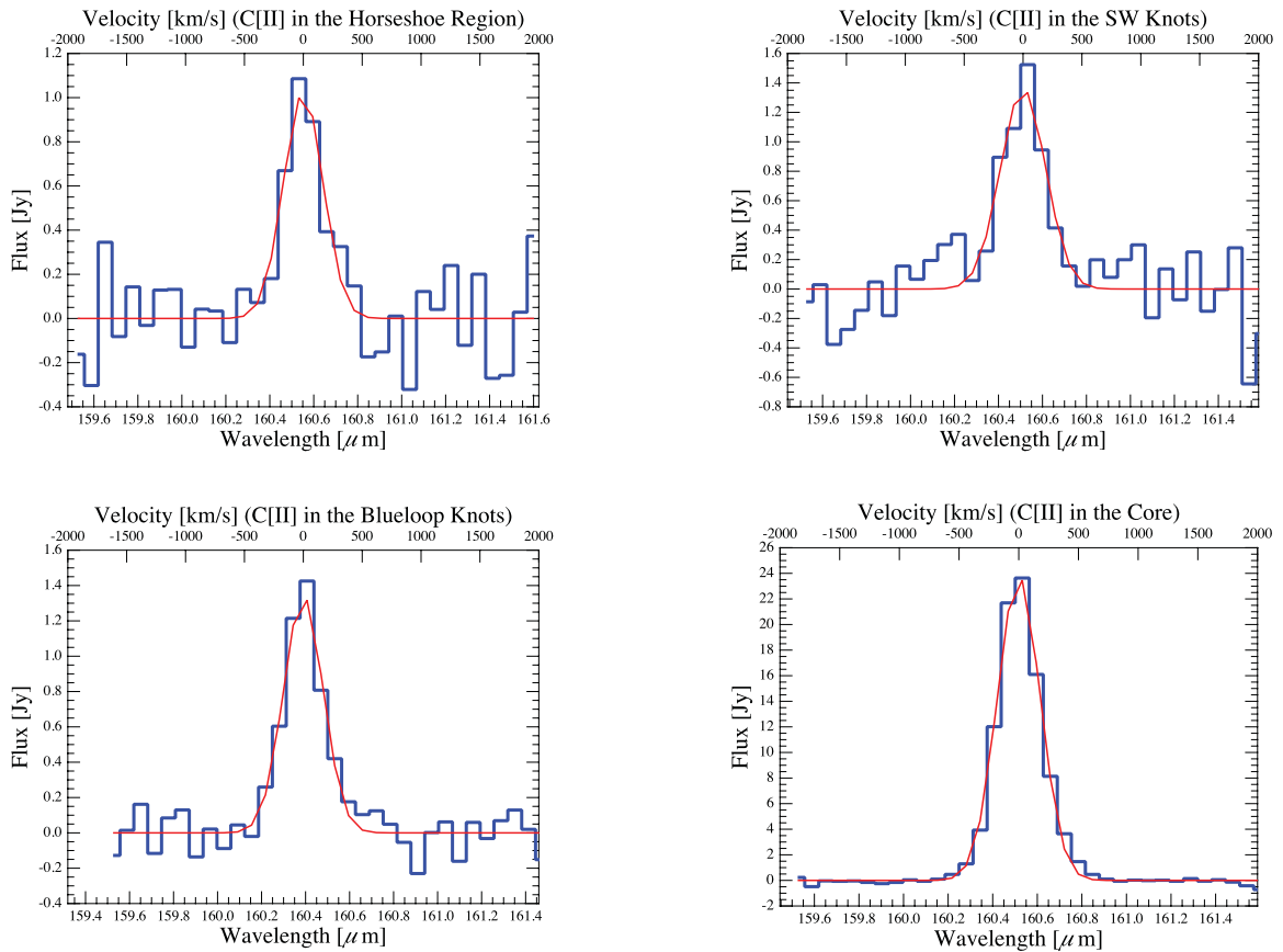
Figure 4. The [C\text{II}] emission from the Horseshoe knot in the NW (upper-left panel), the SW1/SW2 knots in the SW (upper-right panel) and the Blue Loop knots in the SE (lower-left panel). These apertures are marked in Fig. 3. We also show the [C\text{II}] spectrum for the core region (lower-right panel), marked in the upper-left panel of Fig. 5.
