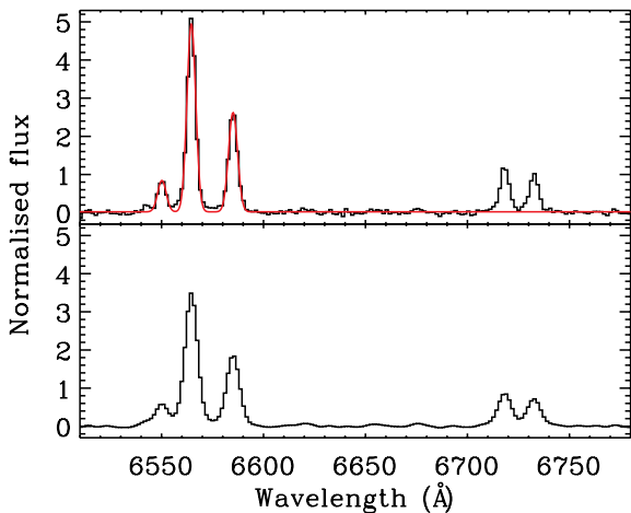
Figure 9. Top: continuum-subtracted narrow emission-line spectrum (black) with the Gaussian fit to the H\alpha and [N II] emission lines overplotted (red). The Gaussian fit has \sigma_{H\alpha} = 98 \text{ km s}^{-1} ( 2.15 \text{ \AA} ). Bottom: the same spectrum after convolving with a Gaussian kernel of width, \sigma_K = 97 \text{ km s}^{-1} , to give an output width of \sqrt{(98 \text{ km s}^{-1})^2 + (97 \text{ km s}^{-1})^2} = 138 \text{ km s}^{-1} .
