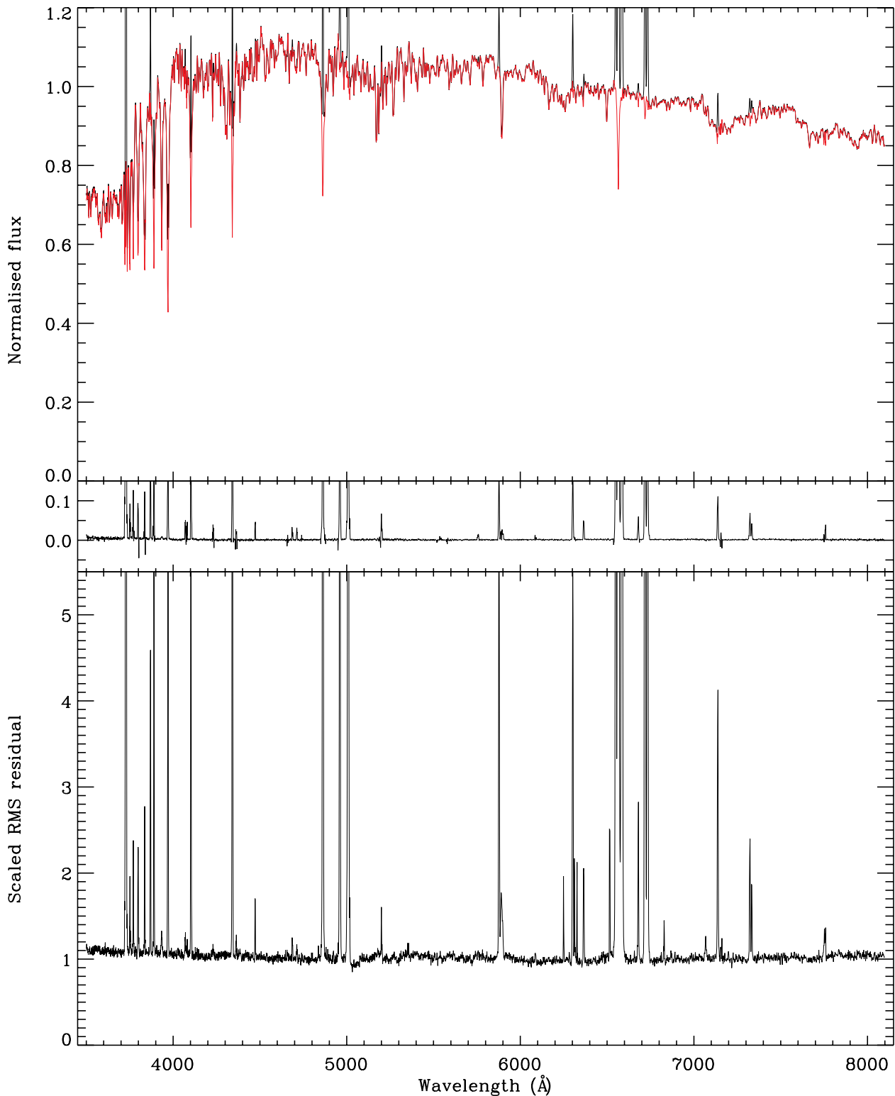
Figure 6. Same as Fig. 3, but for the 727 emission-line galaxies used to generate the emission-line components.
