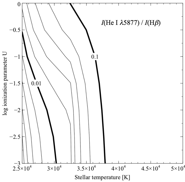
Figure 22. Intensity ratio I(\text{He I } \lambda 5877) / I(\text{H}\beta) for gas photoionized by stellar SEDs, for a range of ionization parameters and stellar effective temperatures.
