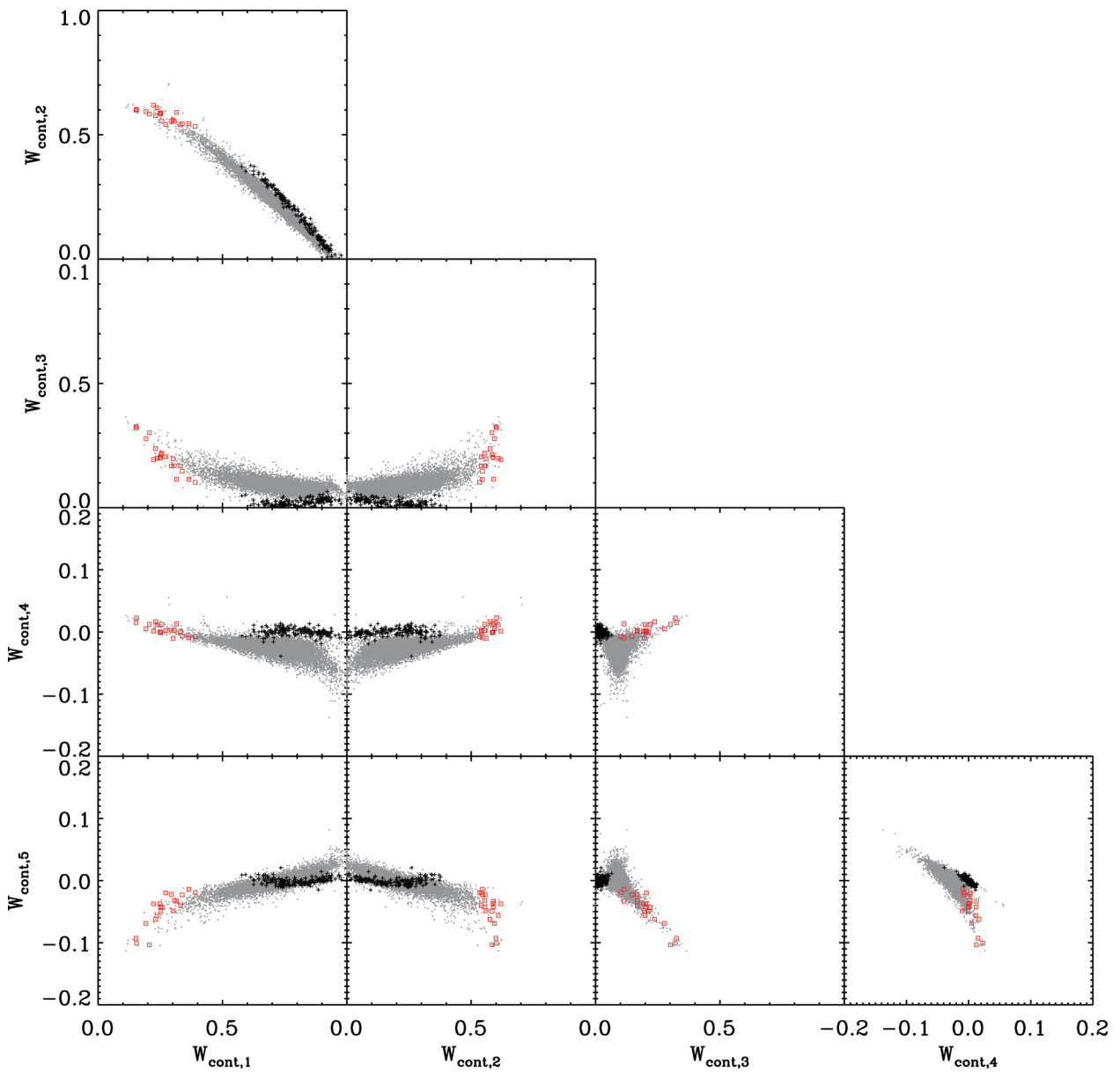
Figure 13. Distributions of continuum component weights. The larger black points are for the 170 galaxies without emission lines; the red squares are for the 20 emission-line galaxies used when generating continuum components 1–3; the smaller grey points are for the full sample of 10 118 emission-line galaxies.
