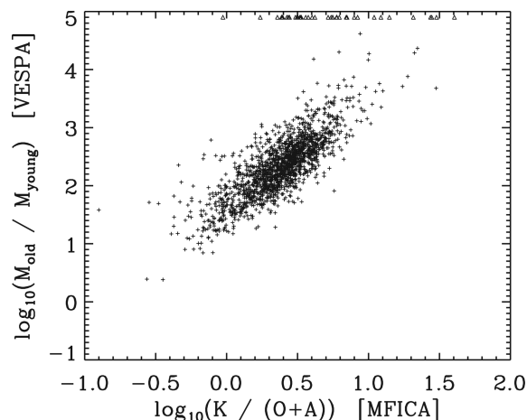
Figure 17. VESPA-derived ratio of old (>0.42 Gyr) to young (<0.42 Gyr) stellar masses, versus ratio of MFICA weights for old (K-giant-dominated) and young (O- and A-star-dominated) stellar populations. Objects beyond the limits of the figure – typically because M_{\text{young}} = 0 – are marked with triangles. Only those galaxies with \tau_V^{\text{ISM}} \leq 0.75 are shown.
