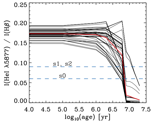
Figure 24. The \text{He I}/\text{H}\beta intensity ratio as a function of starburst age. The thin black lines are for each of the n_{\text{H}}, R points marked by the circles on the bottom-left panel in Fig. 23. The heavy red line is the average of all the thin lines. The horizontal dashed lines show the measured \text{He I}/\text{H}\beta ratios for ICA reconstructions s_0, s_1 and s_2 .
