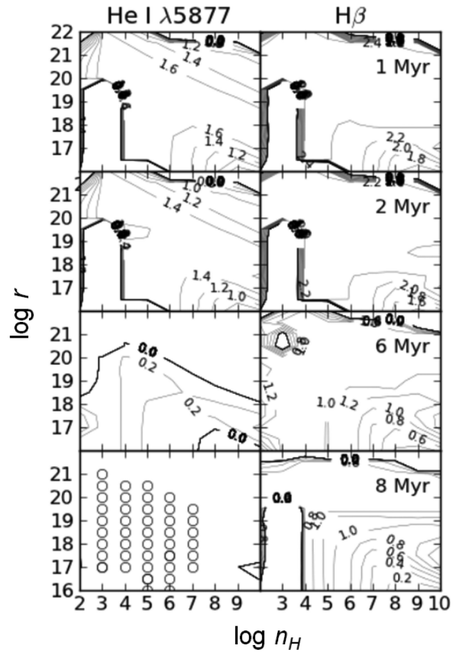
Figure 23. Contour plots showing the EWs of \text{He I } \lambda 5877 and \text{H}\beta emitted by gas clouds as a function of their hydrogen density n_{\text{H}} and their distance R from starbursts of equal ionizing luminosity. The starbursts have different ages, as indicated in the right-hand panel in each row. The circles in the bottom-left panel show the n_{\text{H}}, R values of the curves plotted in Fig. 24.
