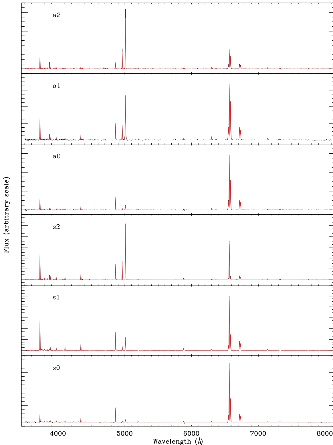
Figure 20. Reconstructed MFICA spectra from a range of positions within the AGN (top three panels) and SF (bottom three panels) loci. In each panel the MFICA reconstruction is in plotted in red, and a composite of the continuum-subtracted spectra of 50 observed galaxies with similar MFICA weights is in black.
