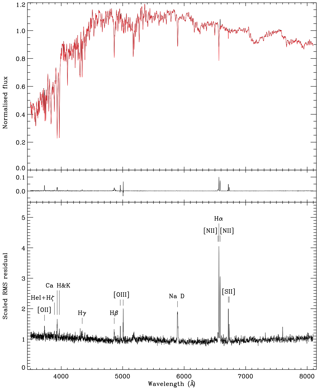
Figure 3. Top: mean normalized spectrum (black) of the galaxies without emission lines, and the corresponding mean MFICA reconstruction (red). Middle: mean residuals after subtracting the MFICA reconstruction. Bottom: rms of the residuals normalized by the SDSS noise arrays. Features corresponding to known emission and absorption lines are labelled. Pixels with zero noise reported in the SDSS spectrum were removed from the rms calculation, as was a strong artefact covering a further four pixels in one of the spectra.
