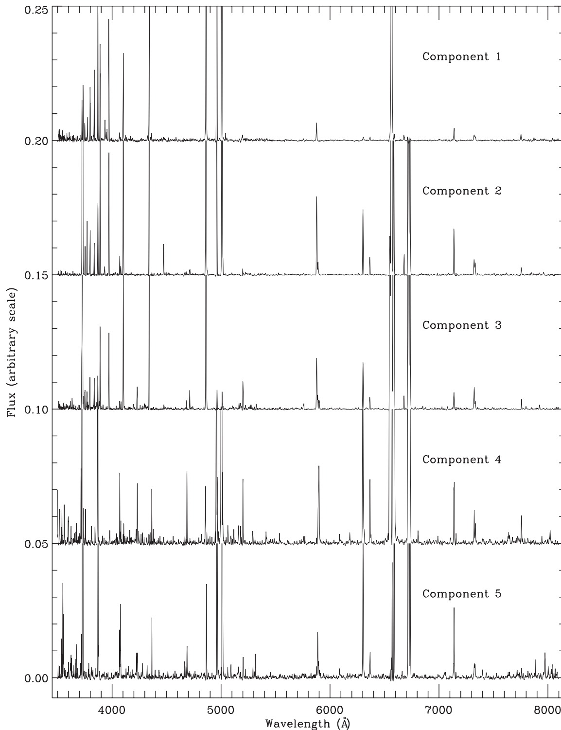
Figure 11. Same as Fig. 10, but showing the faint emission lines. Components are offset for clarity. The ordering of the components and the y-axis scale are the same as in Fig. 10.
