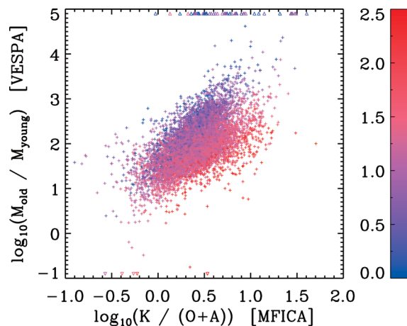
Figure 18. Same as Fig. 17, but showing galaxies with all values of \tau_V^{\text{ISM}} , as denoted by the colour scale. There is a systematic increase in \tau_V^{\text{ISM}} towards the bottom-right corner.
