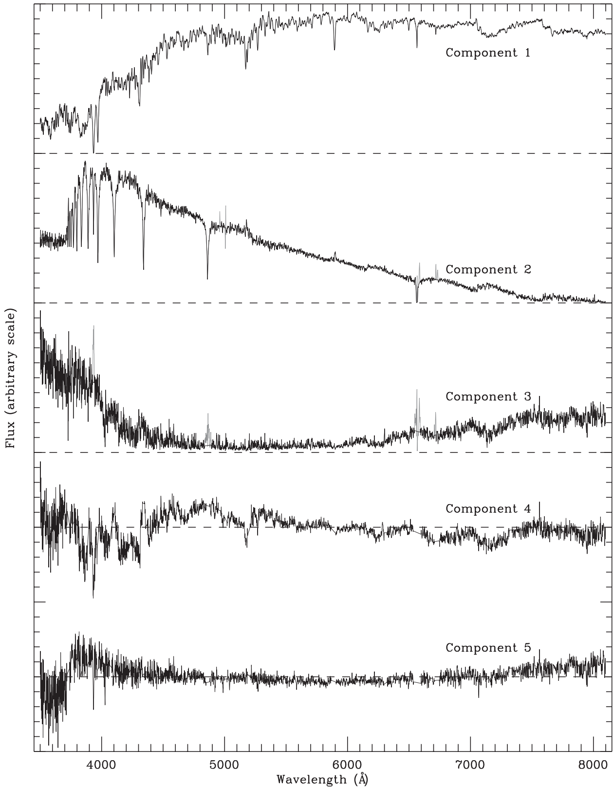
Figure 2. MFICA continuum components. Components are offset for clarity; the dashed lines mark successive zero-points. Components 1–3 were generated from a mixed sample of 170 galaxies without emission lines and 20 with emission lines; the final two ‘adjustment’ components, 4 and 5, were generated from a mixed sample consisting of the same 170 galaxies without emission lines and 727 galaxies with emission lines. For components 1–3, the grey lines show the original components, while the black lines show the final versions after interpolating over a small number of narrow features.
