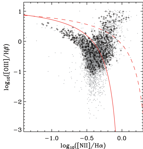
Figure 1. Positions of the input samples in the [\text{O III}] \lambda 5008/\text{H}\beta versus [\text{N II}] \lambda 6585/\text{H}\alpha BPT plane. The small grey points represent the complete emission-line galaxy sample, while the large black points represent those galaxies used to generate the emission-line components. The solid and dashed red lines represent the classification curves defined in Kauffmann et al. (2003) and Kewley et al. (2001), respectively.
