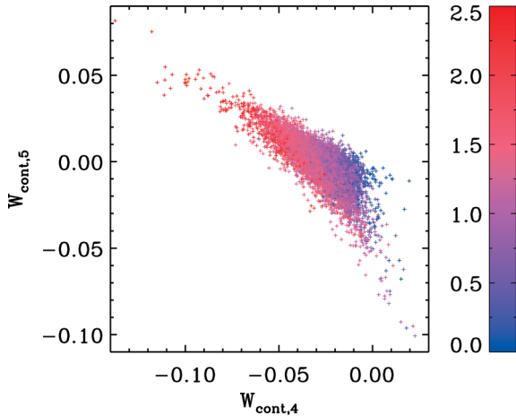
Figure 19. MFICA weights for the two continuum ‘adjustment’ components. Points are colour-coded according to their VESPA-derived \tau_V^{\text{ISM}} value, as in Fig. 18; there is a strong correspondence between \tau_V^{\text{ISM}} and position in the W_{\text{cont},4} – W_{\text{cont},5} plane.
