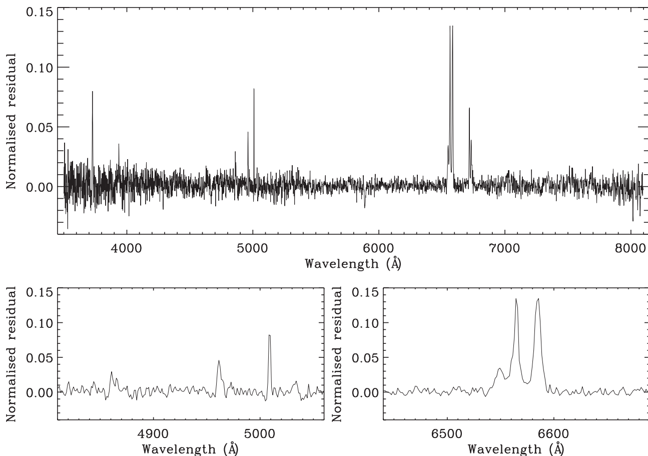
Figure 5. Mean residual spectrum, normalized to the median continuum level, of the 26 per cent of galaxies with the strongest residuals around H\alpha , from the sample without identified emission lines. The lower panels show the regions around H\beta (left) and H\alpha (right) in more detail, showing LINER-like emission-line ratios.
