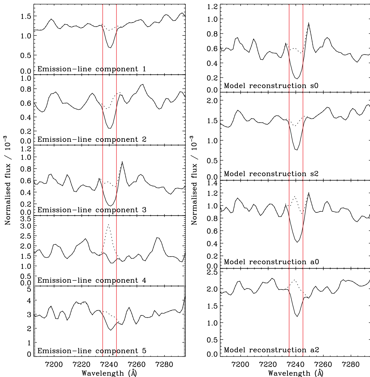
Figure 7. Left: emission-line components (solid lines) generated after an extra mask covering 7235.2\text{--}7245.2\text{ \AA} was included in the continuum component generation. The masked region is shown by vertical red lines. The dotted lines show the median components over all 150 repeats. Right: model spectra (solid lines) formed from the emission-line components shown in the left-hand panels. The median models are shown as dotted lines. The difference between the solid and dotted lines is taken as a measure of the typical error in emission-line flux caused by the masking and interpolation scheme. All components and spectra are normalized relative to their peak flux. No genuine emission lines are seen in the narrow wavelength range plotted.
