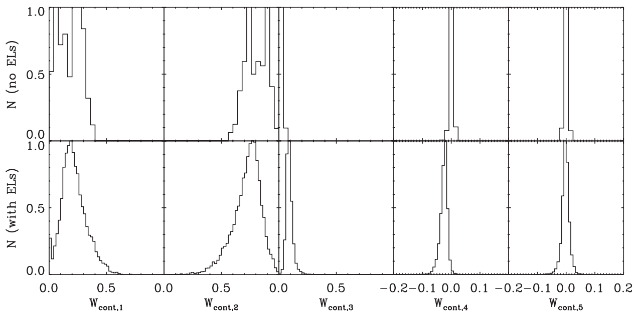
Figure 12. Distributions of the individual continuum component weights, each normalized to their maximum values. The upper panels are for the 170 galaxies without emission lines (ELs), which formed the bulk of the sample from which the first three continuum components were derived. The lower panels are for the full sample of 10 118 emission-line galaxies.
