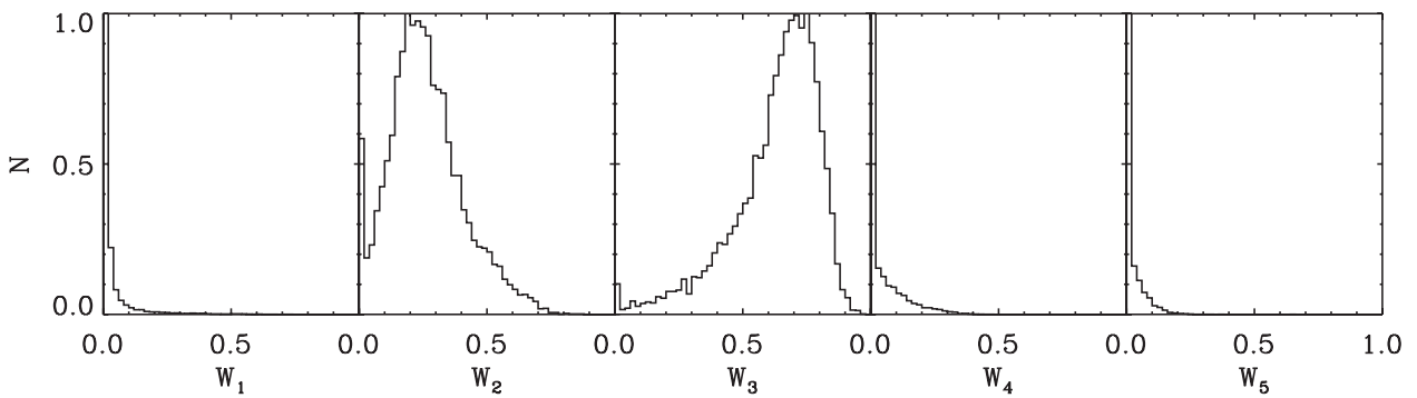
Figure 14. Distributions of the individual emission-line component weights, each normalized to their maximum values.
