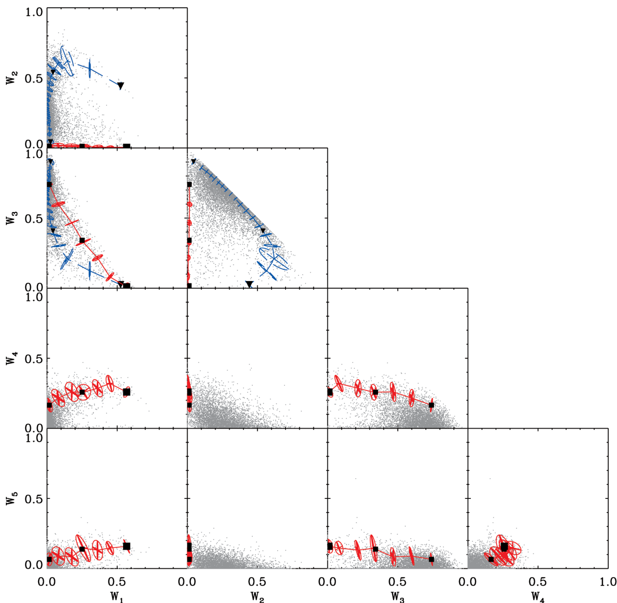
Figure 15. Distributions of emission-line component weights. Overplotted are the loci for SF (dashed blue) and AGN (solid red). The positions of the representative spectra are also shown for SF (triangles) and AGN (squares); the larger symbols represent s2 and a2, i.e. the spectra with the highest [\text{O III}]/\text{H}\beta .
