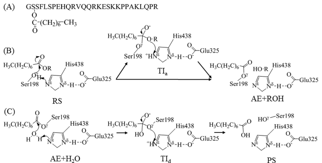
Figure 1. Possible reaction pathways for human BChE-catalyzed hydrolysis of ghrelin. (A) Amino acid sequence of human ghrelin. (B) Acylation process (with or without existence of a tetrahedral intermediate) in which ghrelin is represented as \text{CH}_3(\text{CH}_2)_6\text{COOR} : Reactant State (RS), Tetrahedral Intermediate (TI a ), and Acyl-Enzyme (AE) + desacyl-ghrelin (ROH). (C) Deacylation process: Acyl-Enzyme (AE) + H 2 O, Tetrahedral Intermediate (TI d ), and Product State (PS).
