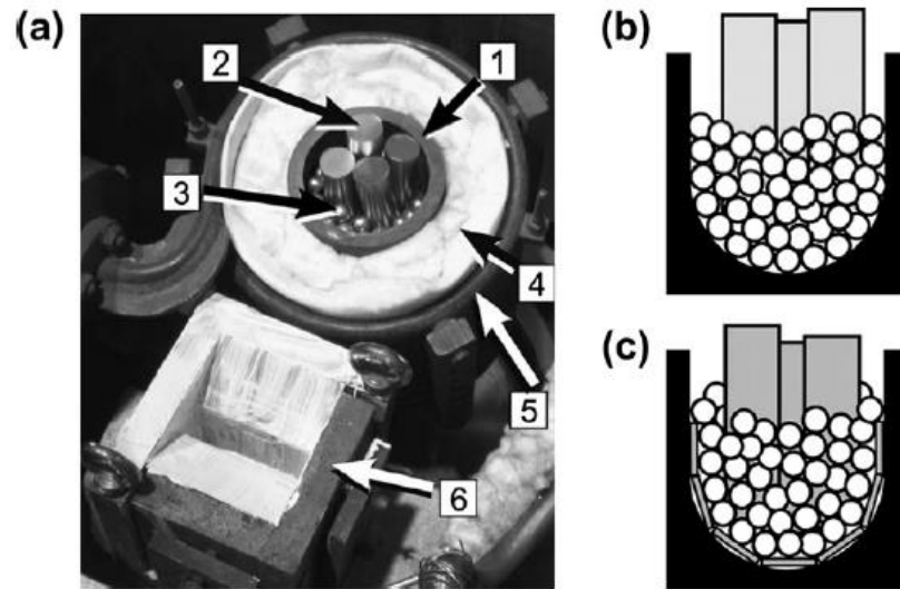
Figure 1-16 (a) Laboratory setup for VIM processing of binary NiTi (1 – graphite crucible; 2 – Ti rods; 3 – Ni pellets; 4 – isolation; 5 --water cooled copper coil; 6 – mold); (b) schematic illustration of the crucible filling with Ni pellets in contact with the graphite [26, 52]
