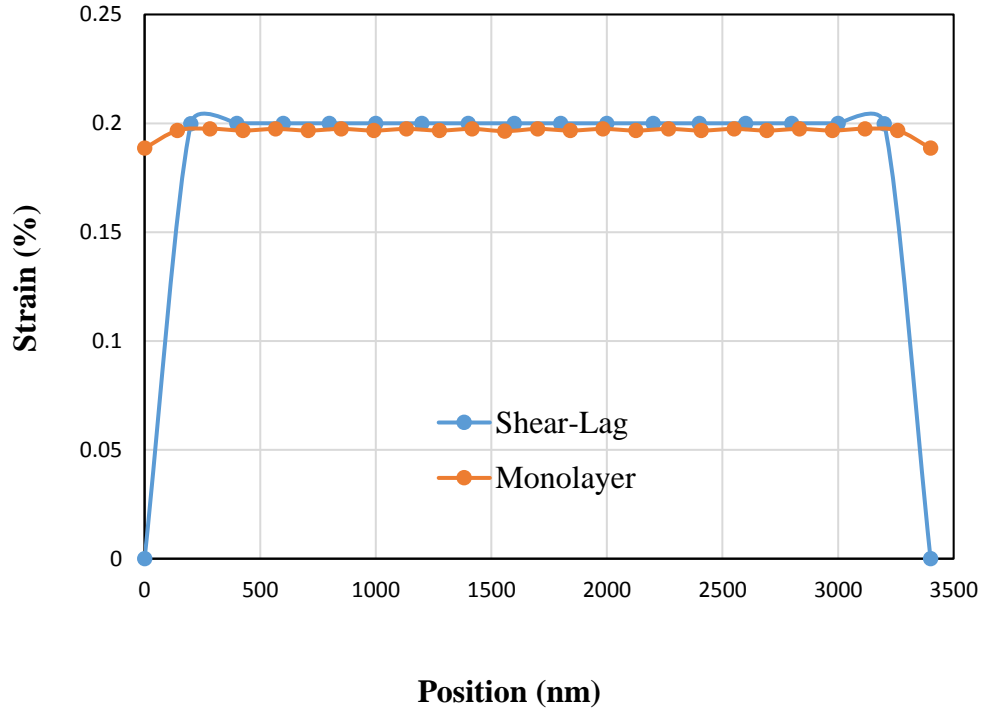
Figure 5.3 Comparison of Monolayer Shear-Lag theory and FEM graphene composite.
