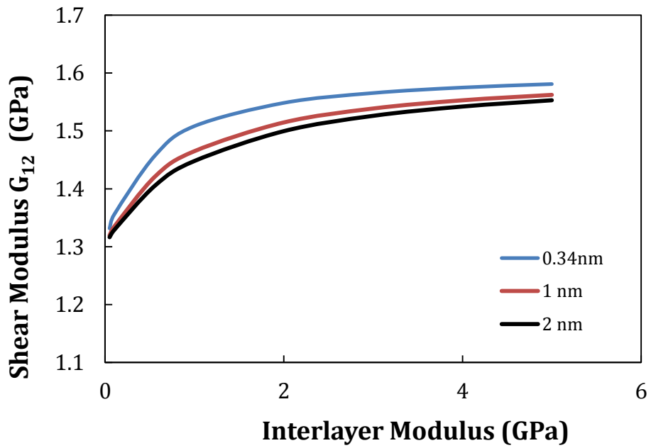
Figure 4.16 Effect of interlayer modulus on effective moduli of layer graphene-polymer composites: out-of-plane shear modulus ( G_{12} ).
