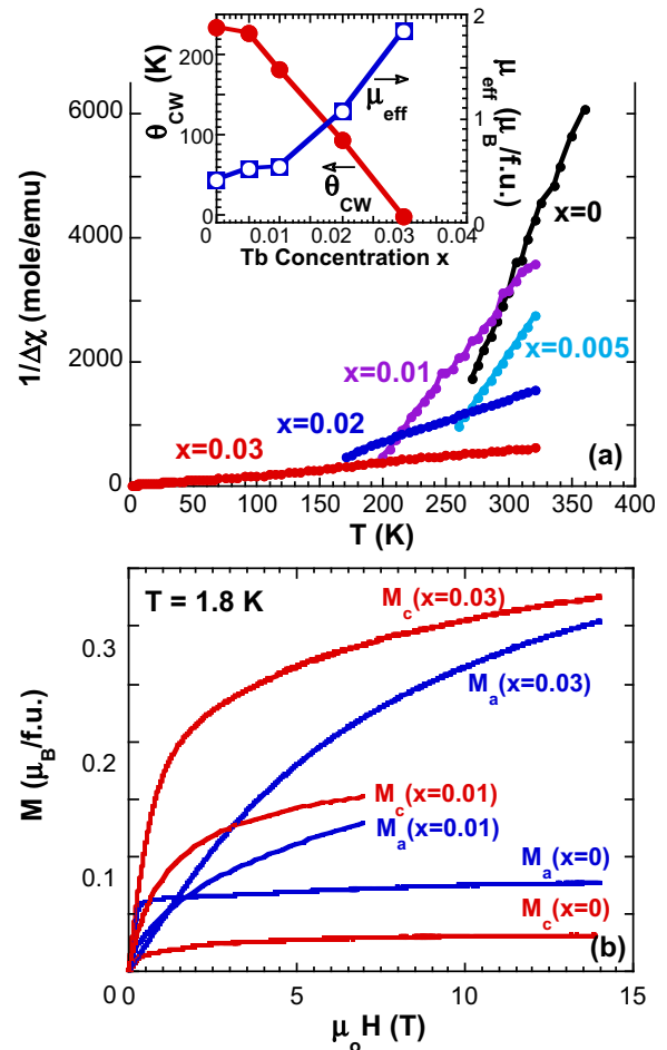
FIG. 5. (Color online) (a) The temperature dependence of \Delta\chi^{-1} for 0 \leq x \leq 0.03 . Inset: The Tb concentration x dependence of the Curie-Weiss temperature \theta_{CW} and effective moment \mu_{eff} . (b) The isothermal magnetization M_a (blue) and M_c (red) up to 14 T for 0 \leq x \leq 0.03 .
