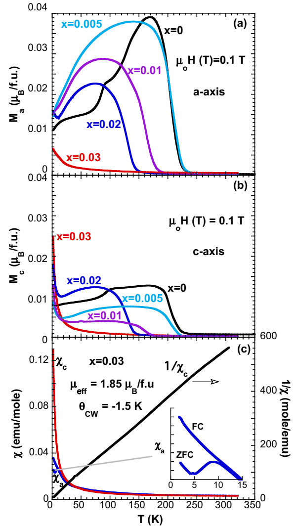
FIG. 4. (Color online) The temperature dependence at \mu_0 H = 0.1 \text{ T} of the magnetization (a) M_a and (b) M_c for 0 \leq x \leq 0.03 ; and (c) \chi_a and \chi_c , and \chi_c^{-1} (right scale) for x = 0.03 . Inset: Enlarged \chi_a for both ZFC and FC samples below 15 K.
