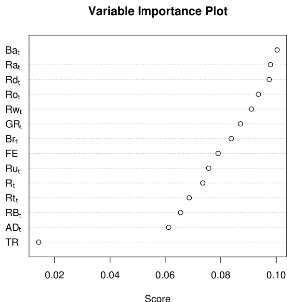
Fig. 5. Variable importance plot for M4_{30} based on the adaptive boosting algorithm.
