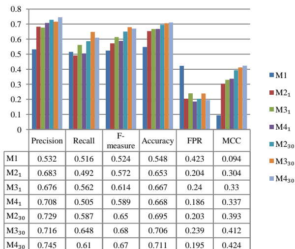
Fig. 4b. RF results for all models.
