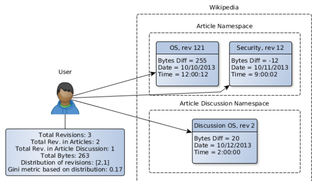
Fig. 1. An example of user activity on Wikipedia along with associated non-verbal activity.
