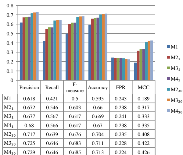
Fig. 4c. ADA results for all models.
