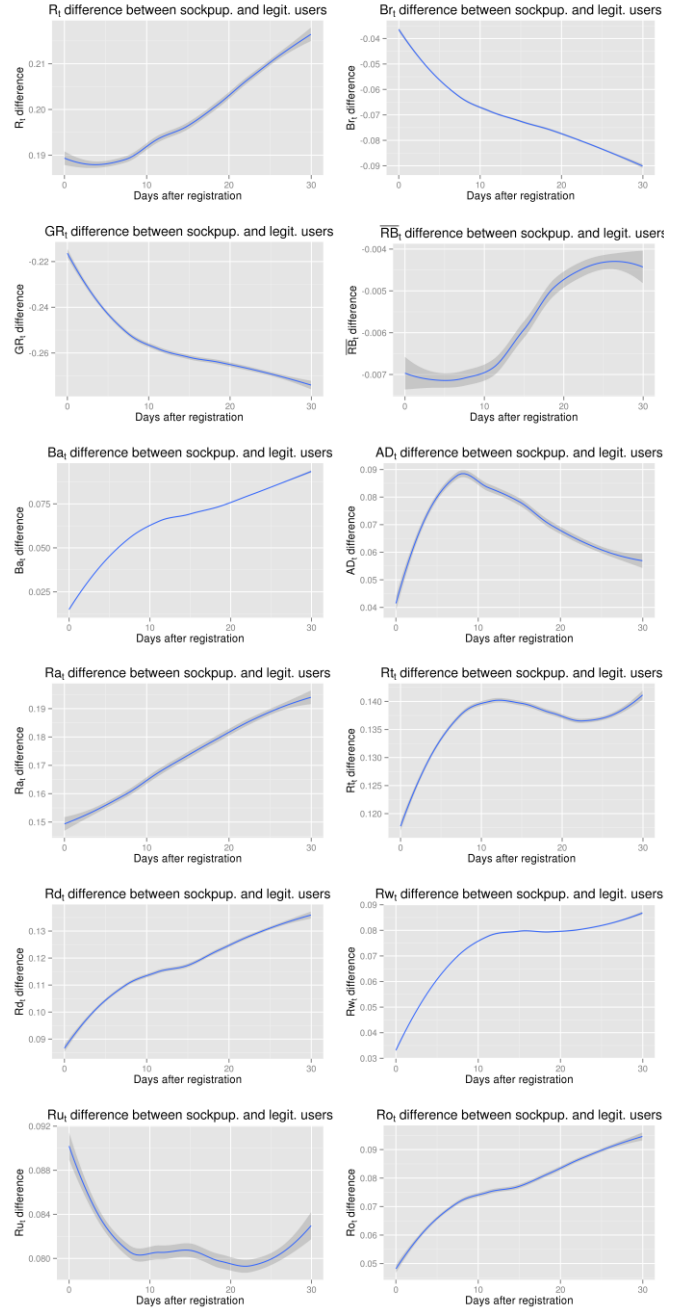
Fig. 3. Variation of differences in non-verbal user activity variables between sockpuppets and legitimate users over a period of a month. Positive scores along the y axis indicate increased activity for sockpuppets whereas negative scores indicate decreased activity for sockpuppets compared to legitimate users.
