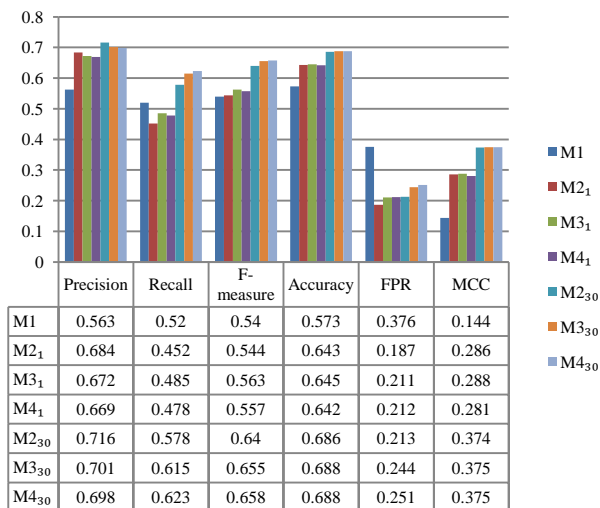
Fig. 4a. SVM results for all models.
