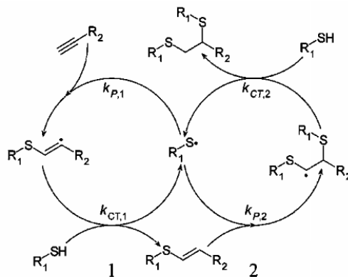
Figure 1.11. Reaction mechanism for addition of thiols to alkynes [102].
