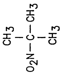
2-Methyl-2-nitropropane
