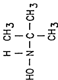
t -Butylhydroxylamine
