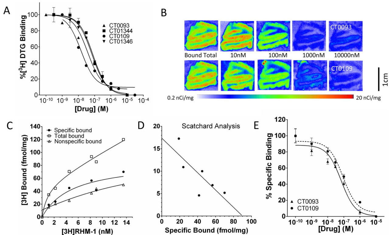
Figure 1. Anti-Abeta compounds are ligands for sigma-2/PGRMC1 receptor. A , CT0109, CT0093, CT01344 and CT01346 displace the fiduciary sigma-2 ligand [ ^3\text{H} ]-DTG from receptors on human B cell lines. B , Autoradiograms of 18.4 nM [ ^{125}\text{I} ]RHM-1 binding to human frontal cortex slices in the presence of 10, 100, 1000, 10,000 nM of CT0109 and CT0093, N=4 . Color bar under images show false coloring scale. [ ^{125}\text{I} ]RHM-1 displays specific saturable binding to human frontal cortex tissue as assessed by quantitative autoradiography in dose-response format ( C ) and as a Scatchard plot ( D ). E , Dose response curves for data obtained from autoradiograms in B . The K_i 's for CT0109 and CT0093 at the [ ^{125}\text{I} ]RHM-1 binding site were 57 \pm 23 nM and 33 \pm 12 nM, respectively. doi:10.1371/journal.pone.0111899.g001
