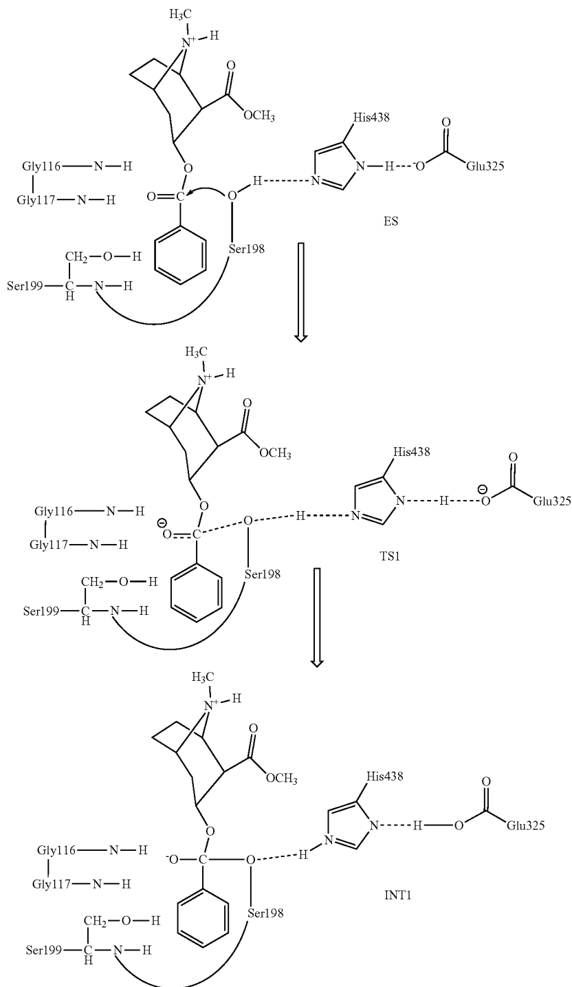
Scheme 4. Schematic representation of the first reaction step for (-)-cocaine hydrolysis catalyzed by a BChE mutant with an A199S mutation.
