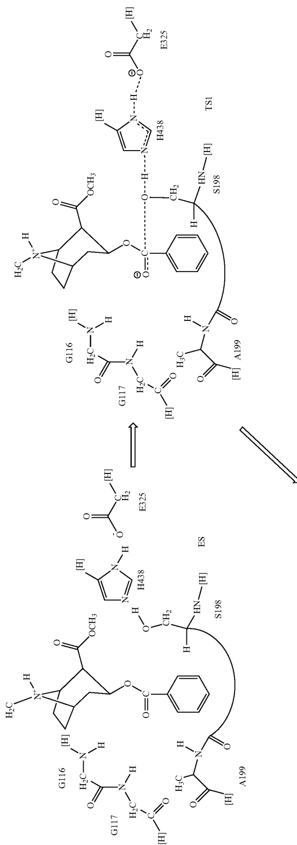
Scheme 3. Schematic representation of BChE-catalyzed hydrolysis of (-)-cocaine. Only QM-treated high-layer part of the reaction system in QM/MM calculations are drawn. Notation [H] refers to a non-hydrogen atom in the MM-treated low-layer part of the protein and the cut covalent bond with this atom is saturated by a hydrogen atom. The dash lines in the transition state structures represent the transition bonds.
