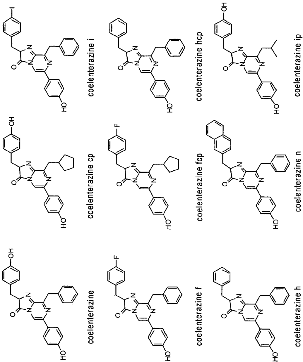
Fig. 16 Coelenterazine Analogs
