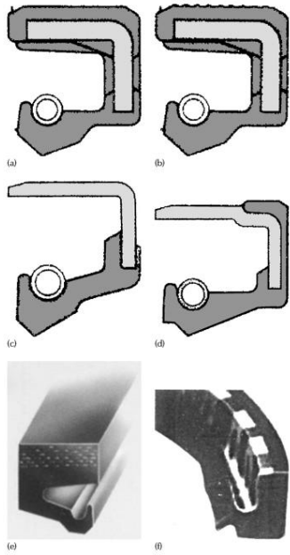
Figure 3.2. Examples of lip seal casing designs: (a) elastomer covered casing; (b) ribbed elastomer coating; (c) metal casing; (d) metal casing with partial elastomer sleeve on the o.d. to provide improved retention; (e) elastomer fabric casing that is used instead of metal on some large diameter seals; (f) complete elastomer seal with U section finger spring. (Source: (a)–(d) Freudenberg Simrit, (e) James Walker, (f) Garlock Kleaire)
