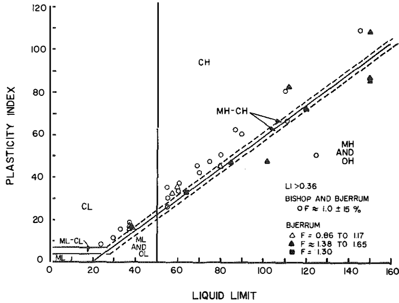
Figure 14. Plasticity Chart Showing the Atterberg Limits of Slope Failures in Normally Consolidated Clays (data from Bishop and Bjerrum (14), Bjerrum (8), and Kentucky DOT Division of Research). The liquidity index for these cases was greater than 0.36. Factor of safety for these cases was within 1.0 \pm 15 percent, except for seven cases of Bjerrum's data where the safety factor ranged from 1.38 to 1.65.
