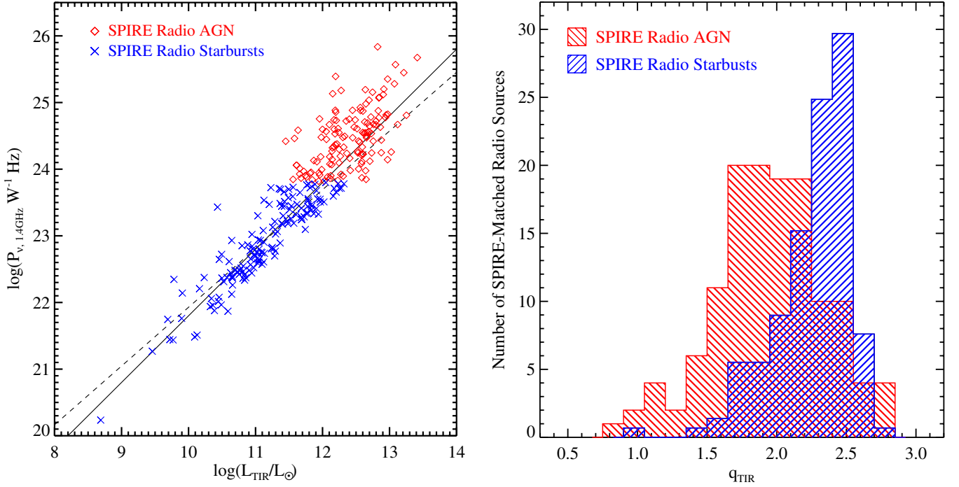
Fig. 4. Left: total infrared (TIR) luminosity plotted against the rest-frame power density at 1.4 GHz of all galaxies with reliable redshifts detected significantly in both the VLA and Herschel imaging. Galaxies which we have defined as hosting radio AGN are represented by open red diamonds and galaxies whose radio emission likely originates either solely from star-forming processes or some combination of star formation and AGN activity are shown as blue Xs. The dashed line denotes our formal best fit relation for SPIRE radio starbursts. The solid line is the best-fit relation from Del Moro et al. (2013) for “radio normal” galaxies. Right: histogram of q_{\text{TIR}} for the SPIRE radio AGN and SPIRE radio starburst samples. The two histograms are normalized to each other. Though there is significant overlap between the two samples, in large part due to SPIRE radio starbursts that likely host lower luminosity AGN, the two distributions are inconsistent with being drawn from the same parent sample.
