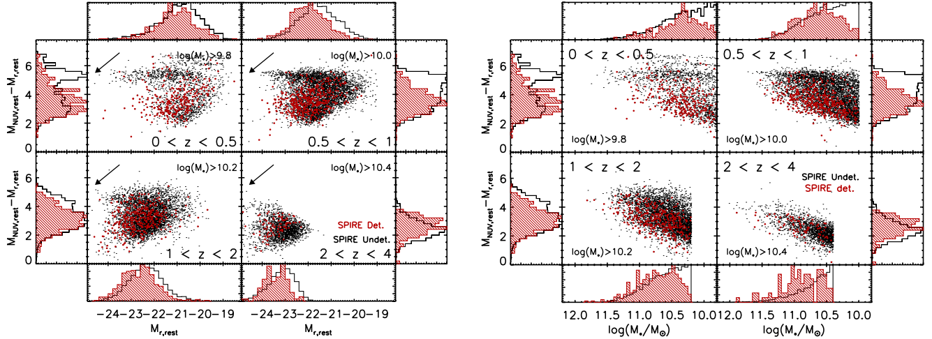
Fig. 7. Rest-frame M_{NUV} - M_r color magnitude ( left ) and color stellar mass ( right ) diagrams of the full SPIRE sample (filled red circles and dashed red histograms) and galaxies undetected in SPIRE (small black points and open black histograms). Galaxies are binned into four different redshift bins and histograms of each sample are normalized (such that the maximal value is unity) for each redshift bin. Only those galaxies detected at high significance in CFHT-WIRDS K_s -band imaging are shown in both panels. In each panel the sample is restricted to those galaxies with stellar masses above the stellar mass limit for each redshift range (given in each panel). The arrow denotes the change in color and (where appropriate) absolute magnitude for an extinction value of E_s(B - V) \sim 0.3 using a Calzetti et al. (2000) extinction law. The arrow is vertical in the right panel because the measured extinction values are already incorporated into the SED-fitting process. The SPIRE-detected sample spans the full range of absolute magnitudes, stellar masses, and, surprisingly, colors in each redshift bin.
