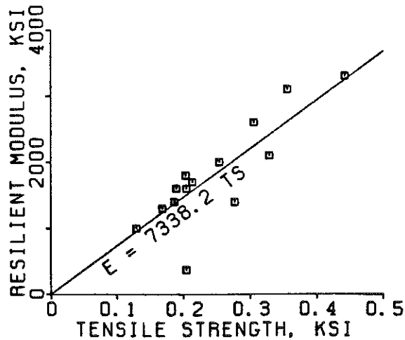
Figure 4. Resilient Modulus as a Function of Splitting Tensile Strength.
