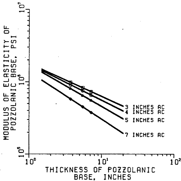
Figure 10. Equivalent Thickness Designs Using Pozzolanic Base for Varying Thicknesses of Asphaltic Concrete and Moduli of Pozzolanic Base Materials.
