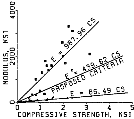
Figure 3. Modulus of Elasticity versus Compressive Strength for Various Data Sources.
