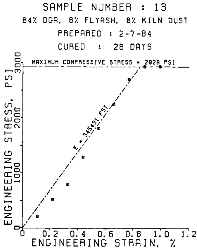
Figure 2. Example Determination of Static-Chord Modulus.
