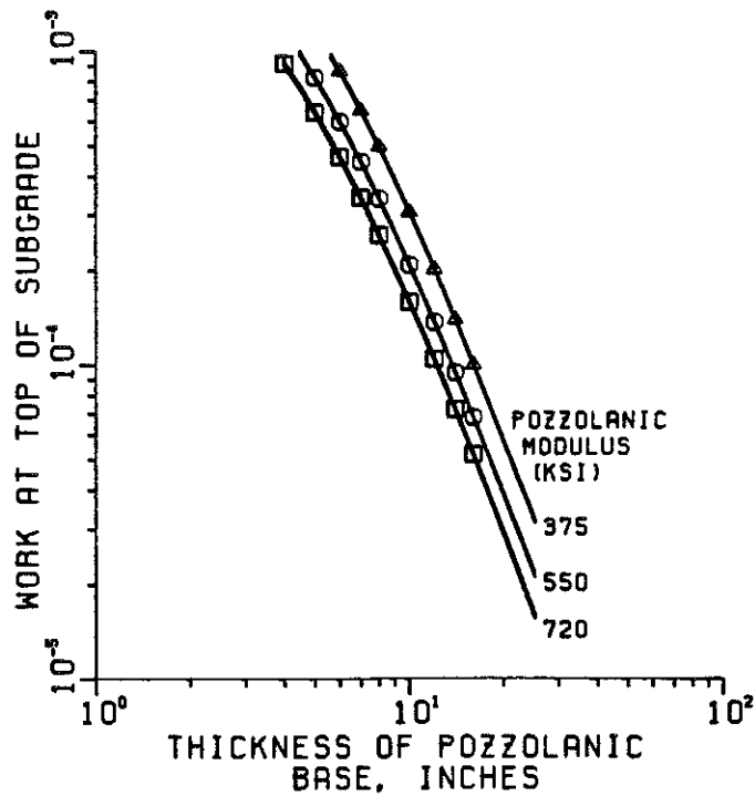
Figure 9. Work at Top of Subgrade versus Thickness of Pozzolanic Base for Constant Modulus of Elasticity of Pozzolanic Base and Constant Thickness of Asphaltic Concrete Surfacing.
