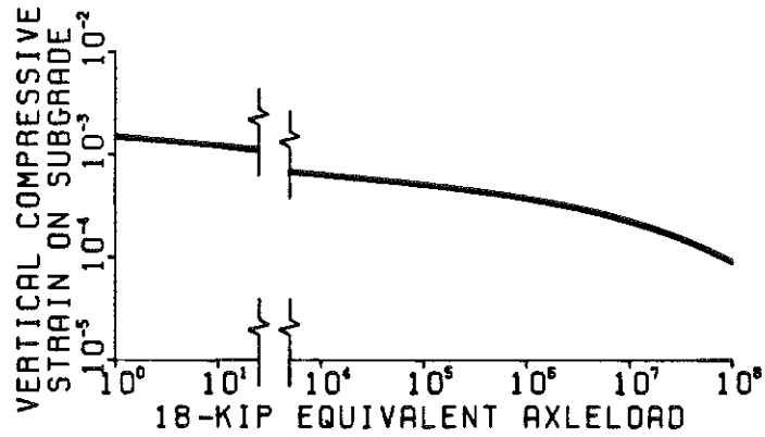
Figure 5. Limiting Subgrade Vertical Compressive Strain versus Repetitions of an 18,000-pound Axleload.
