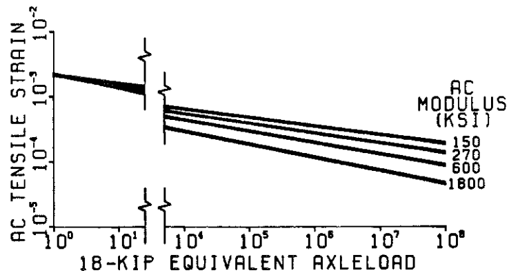
Figure 6. Limiting Tensile Strain at Bottom of the Asphaltic Concrete versus Repetitions of an 18,000-pound Axleload.
