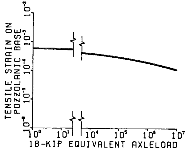
Figure 7. Limiting Tensile Strain at Bottom of the Pozzolanic Base versus Repetitions of an 18,000-pound Axleload.
