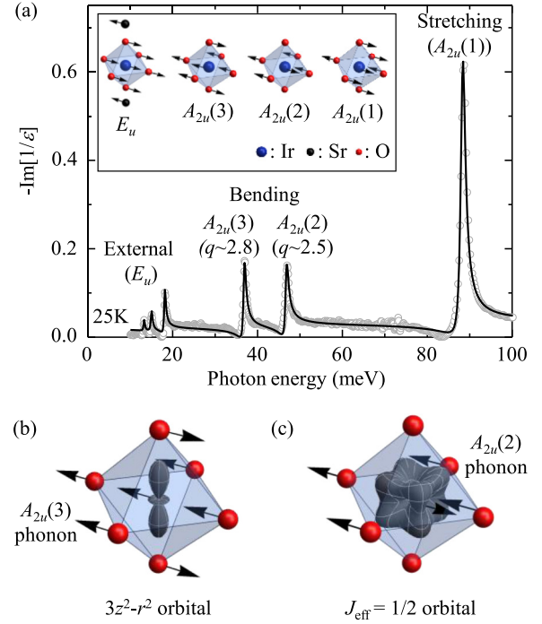
FIG. 3. (Color online) (a) -\text{Im}(1/\epsilon) of \text{Sr}_2\text{IrO}_4 taken at 25 K. The six sharp peaks correspond to LO phonon modes. Each phonon mode is illustrated in the inset. Schematics of the formation of polarons in the cases of (b) 3z^2-r^2 electrons and (c) J_{\text{eff}} = 1/2 electrons.
