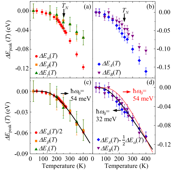
FIG. 2. (Color online) \Delta E_{\text{peak}}(T) for (a) peaks \alpha , \beta , and \gamma , and (b) peaks A and B. (c) \Delta E_{\alpha}(T)/2 , \Delta E_{\beta}(T) , and \Delta E_{\gamma}(T) , which represent \Sigma'(T) of J_{\text{eff}} = 1/2 electrons. The black thick line is the best fitting result with the Fröhlich polaron model. (d) \Delta E_A(T) - \frac{1}{2}\Delta E_{\alpha}(T) and \Delta E_B(T) , which represent \Sigma'(T) of 3z^2-r^2 electrons. The black thick line is the best fitting result with the polaron model, while the red thin line is the fitting line with 54 meV phonon energy for comparison.
