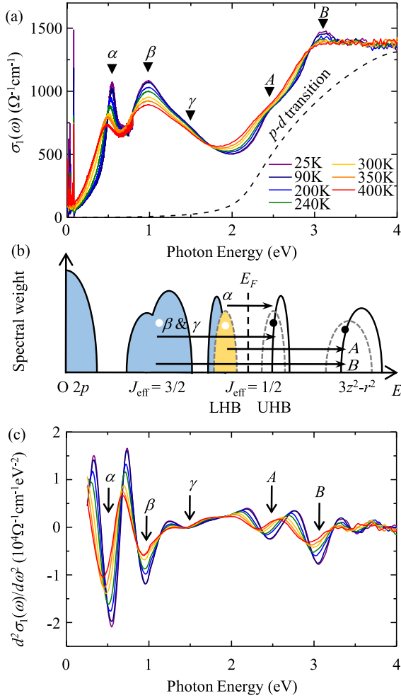
FIG. 1. (Color online) (a) T -dependent \sigma_1(\omega) of \text{Sr}_2\text{IrO}_4 . The black dashed line indicates the contribution of broad p - d transitions. Five sharp electronic transitions are indicated by \alpha , \beta , \gamma , A, and B, in order of increasing energy. (b) Schematic diagram of the optical transition and spectral weights in \text{Sr}_2\text{IrO}_4 . The solid (dashed) line represents the spectral weights in a noninteracting (interacting) system. (c) Second derivatives of \sigma_1(\omega) , d^2\sigma_1(\omega)/d\omega^2 . The black arrows indicate the dips in d^2\sigma_1(\omega)/d\omega^2 , corresponding to the peak energies in \sigma_1(\omega) .
