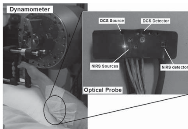
Fig. 1 Experimental setup showing dynamometer and flexible fiber-optic probe containing source and detector fibers for both NIRS and DCS, taped to forearm flexor muscles (flexor digitorum superficialis/profundus). Subject is supine, while arm is slightly elevated on a pillow. Hand is resting around handgrip attachment of the dynamometer.
