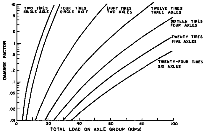
Figure 1. Damage (or Load Equivalency) Factor for Selected Axle Groups as a Function of Load on the Axle Group.
