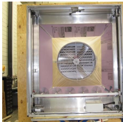
Figure 4-14 – Fan testing setup; treatment 36_54_60D
