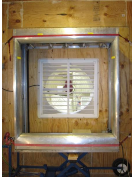
Figure 4-6 – Fan testing setup; Treatment 36_48_I
