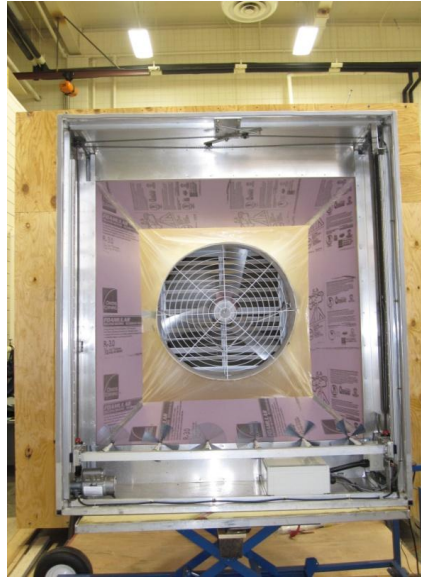
Figure 4-13 – Fan testing setup; treatment 36_54_45D
