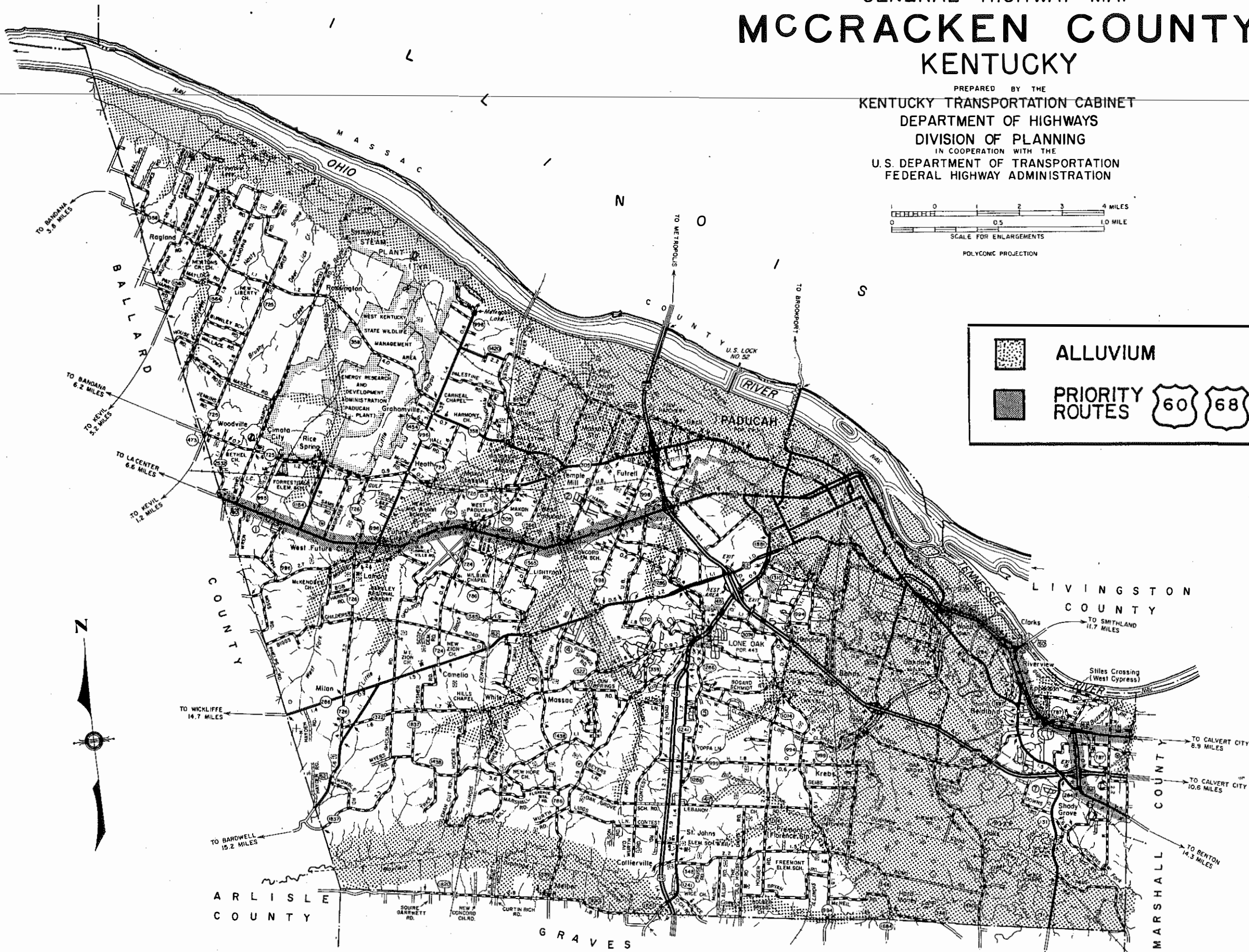
Figure 3. Alluvium map for McCracken County.
