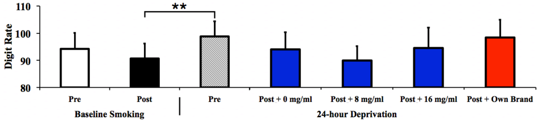
Figure 3a: Rapid Information Processing Task: Digit Rate
